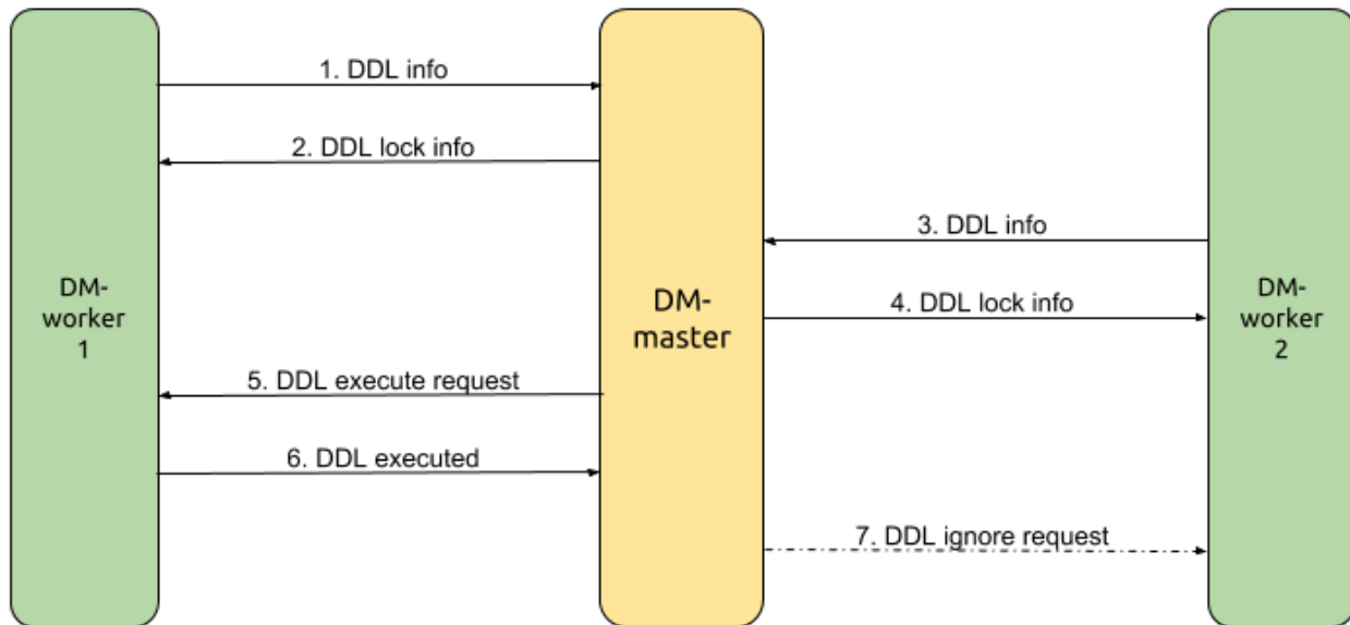
Figure 3: shard-ddl-flow
