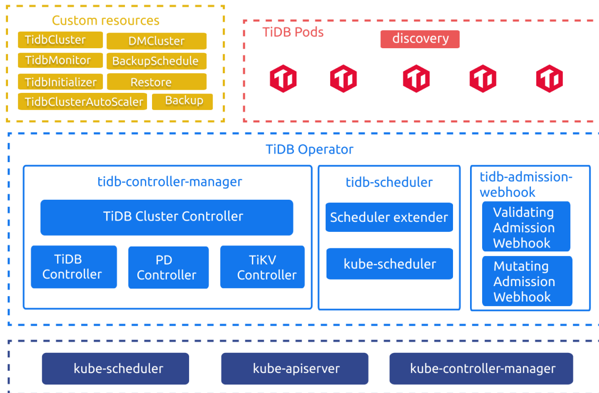
Figure 6: TiDB Operator Overview
