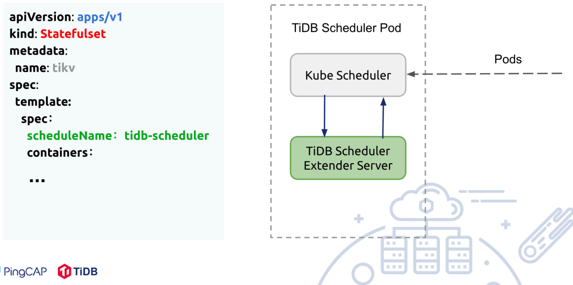
Figure 8: TiDB Scheduler Overview
