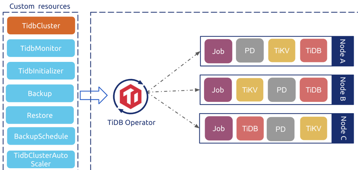
Figure 7: TiDB Operator Control Flow
