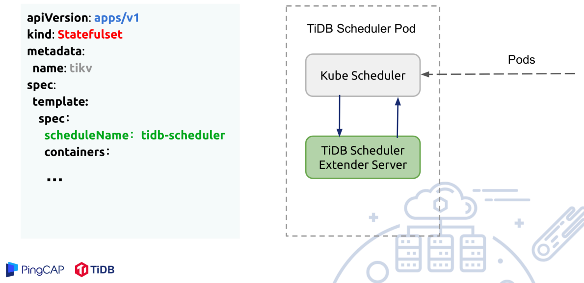
Figure 8: TiDB Scheduler Overview
