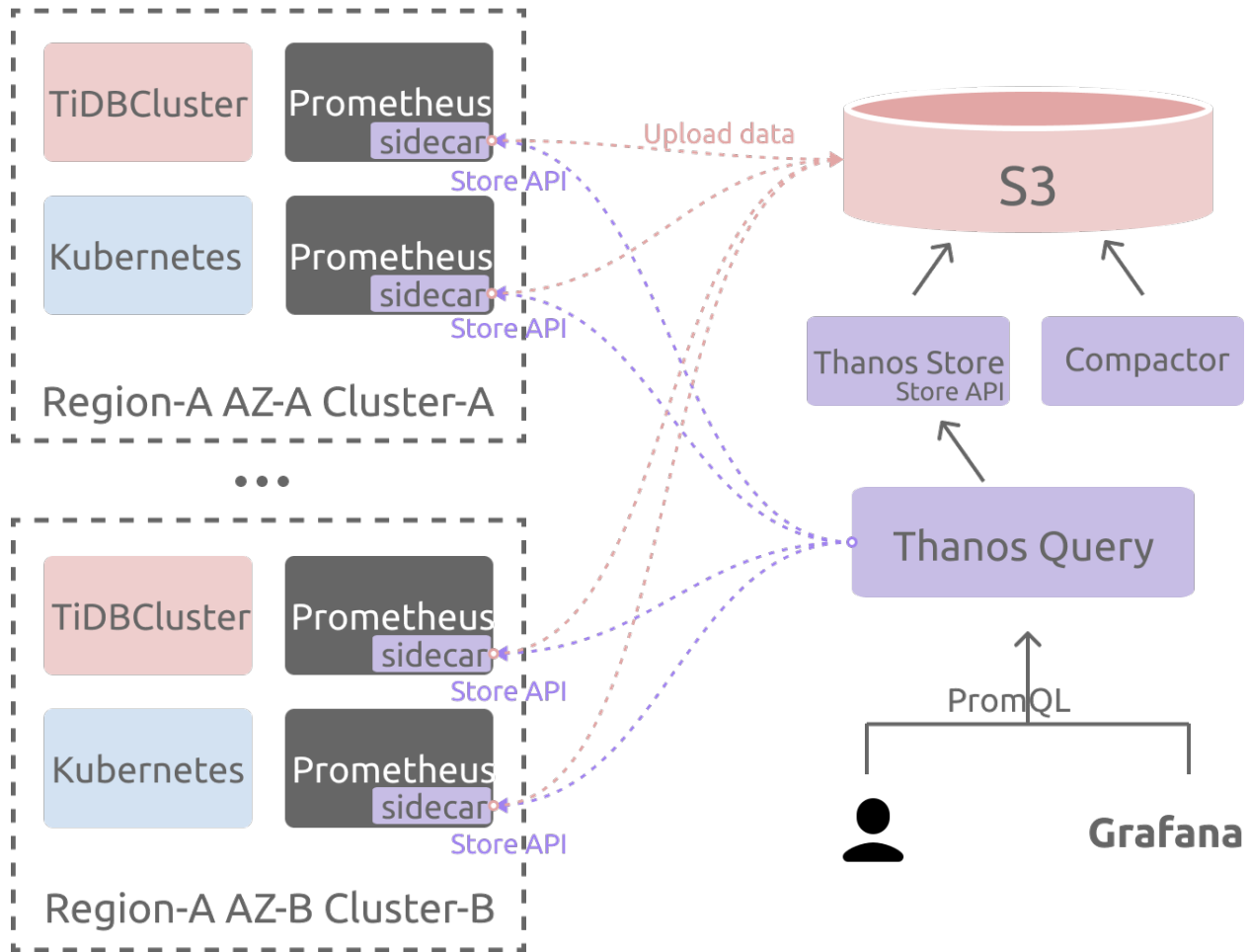
Figure 3: pull-thanos-query.png
