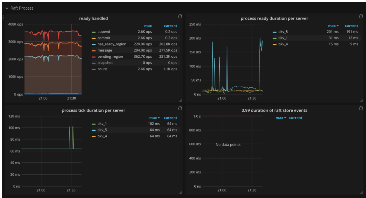
图 235: TiKV Dashboard - Raft process metrics
