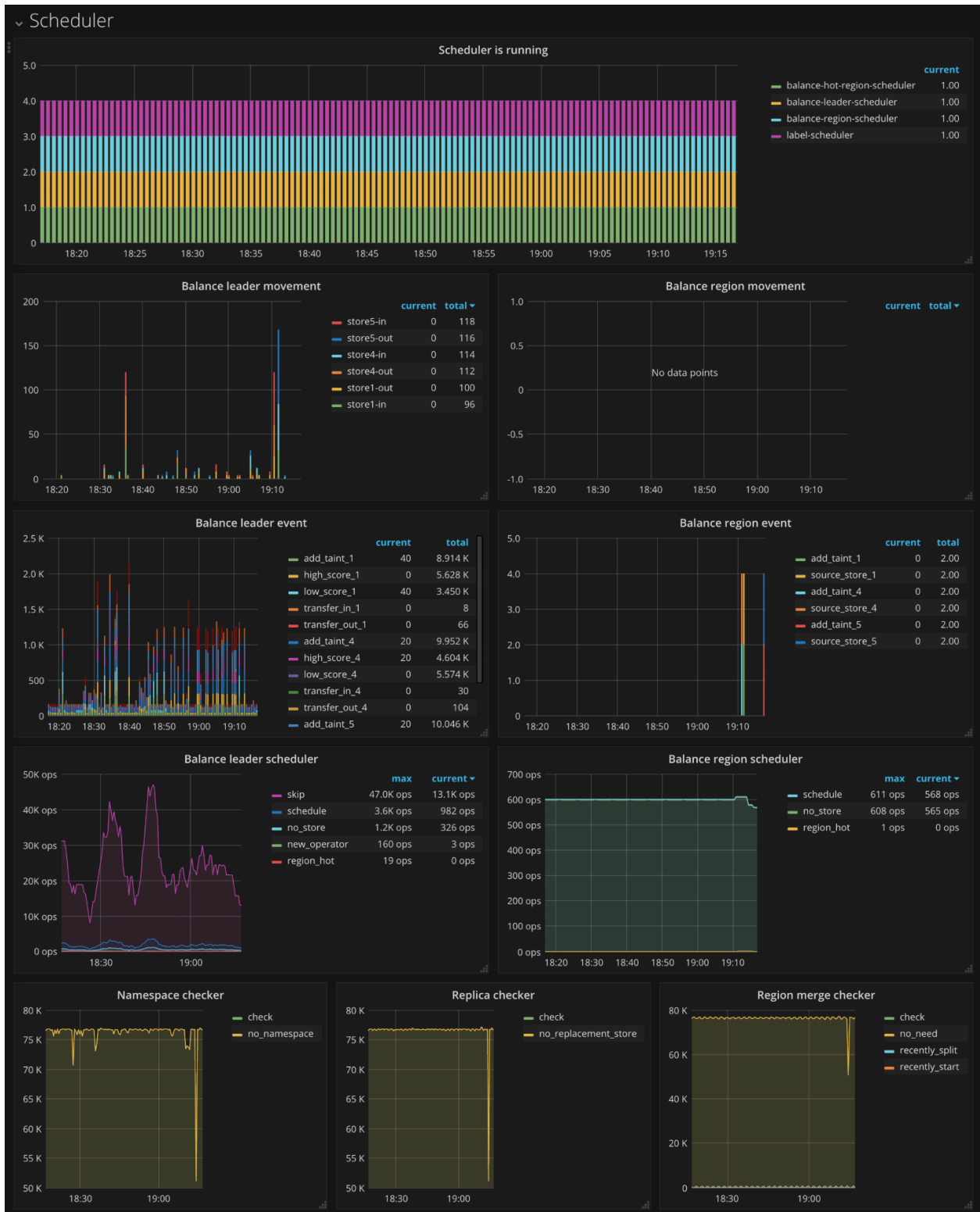
225: PD Dashboard - Scheduler metrics
