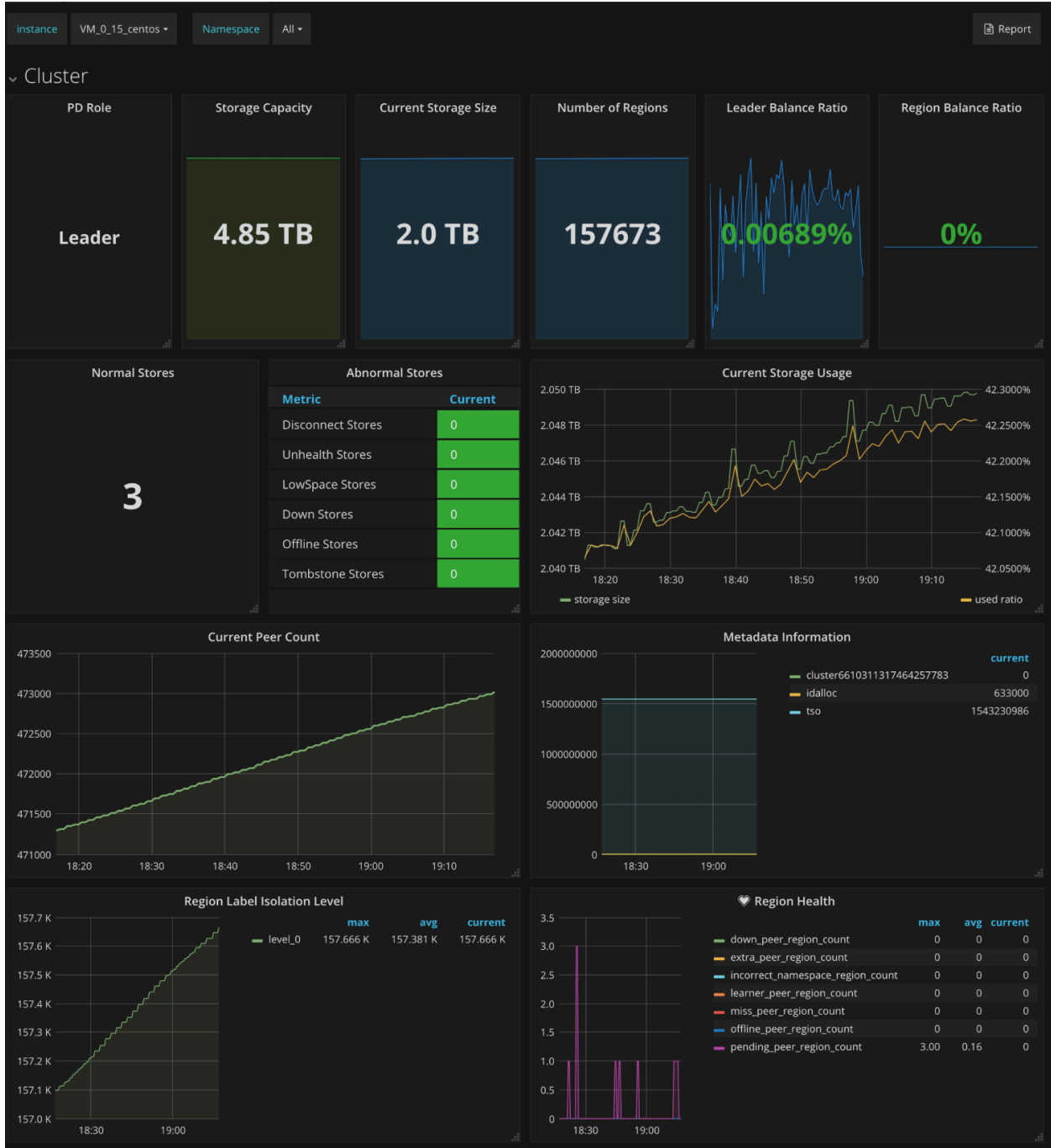
图 222: PD Dashboard - Cluster metrics
