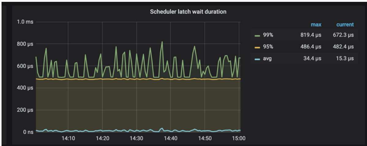
图 220: Scheduler latch wait duration
