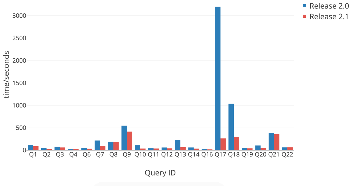
图 7: TPC-H Query Result
