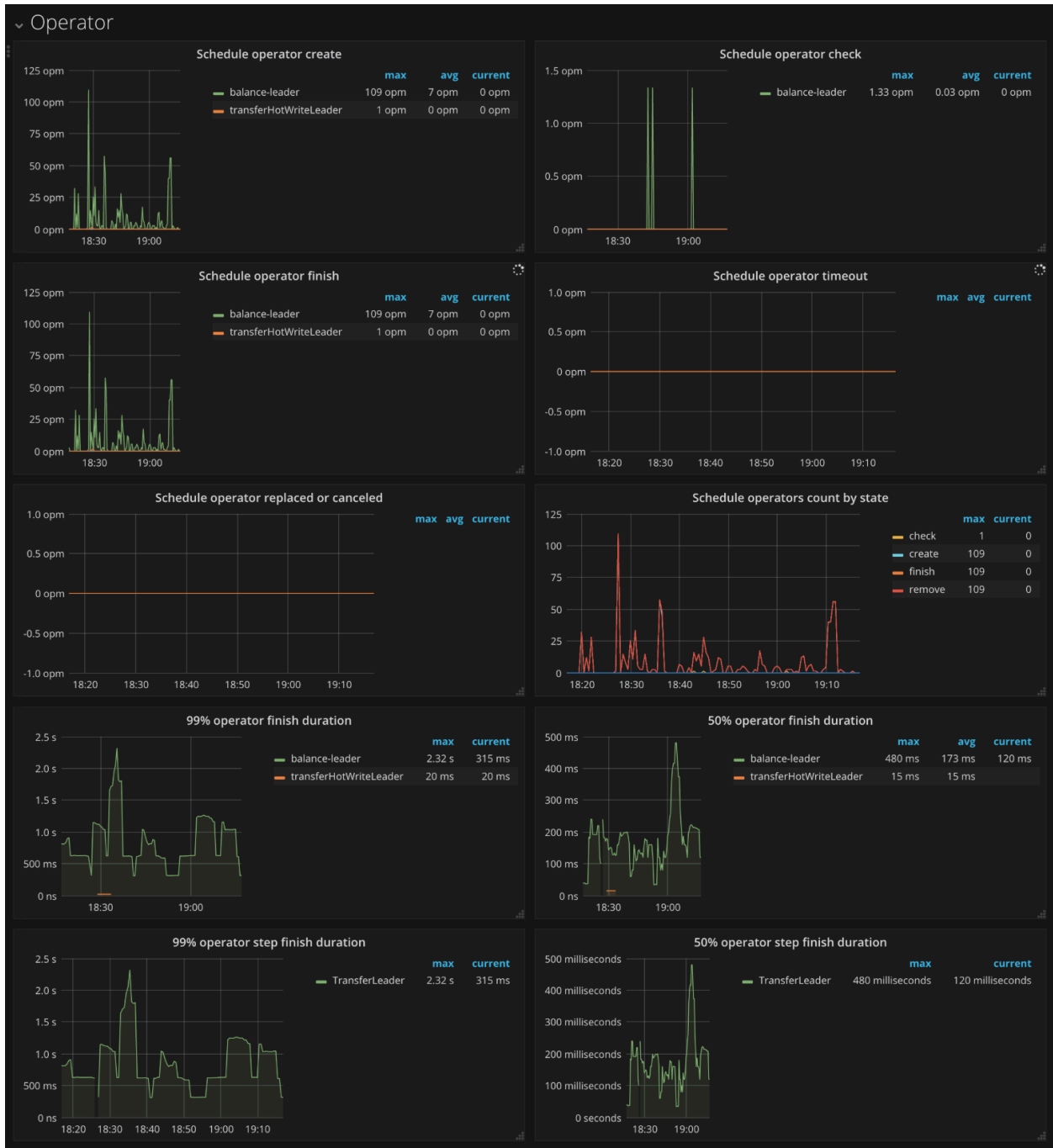
图 226: PD Dashboard - Operator metrics
