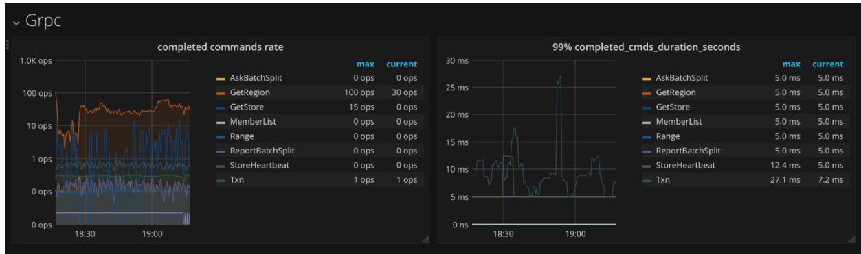
图 227: PD Dashboard - gRPC metrics
