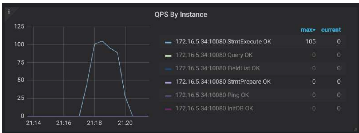
图 247: QPS By Instance
