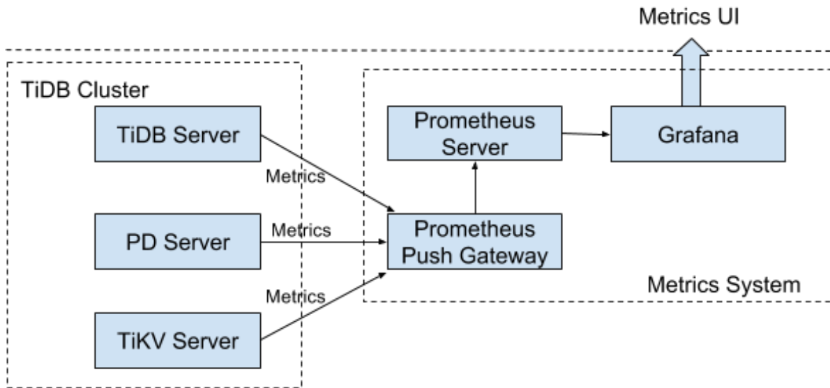
图 20: Deployment Architecture
