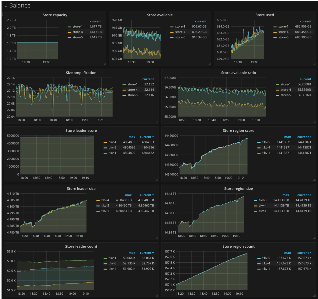
图 223: PD Dashboard - Balance metrics
