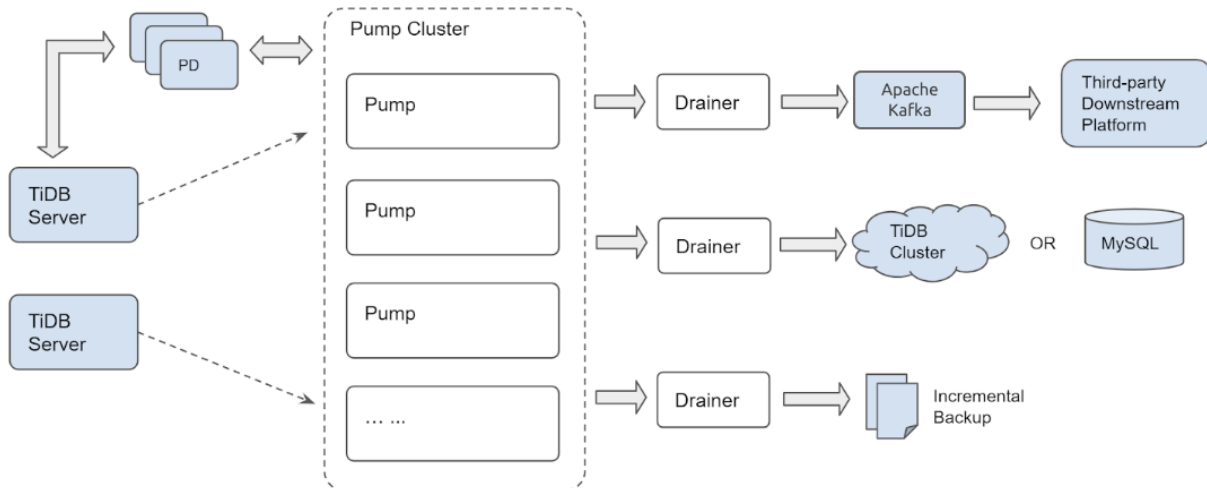
图 9: TiDB Binlog architecture
