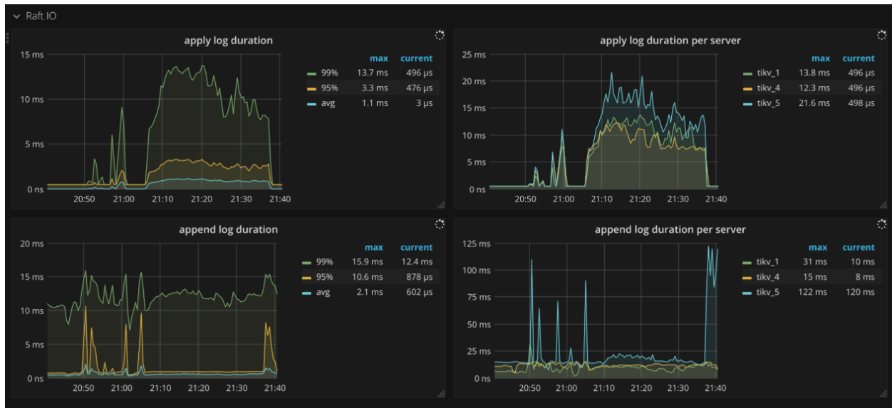
图 234: TiKV Dashboard - Raft IO metrics
