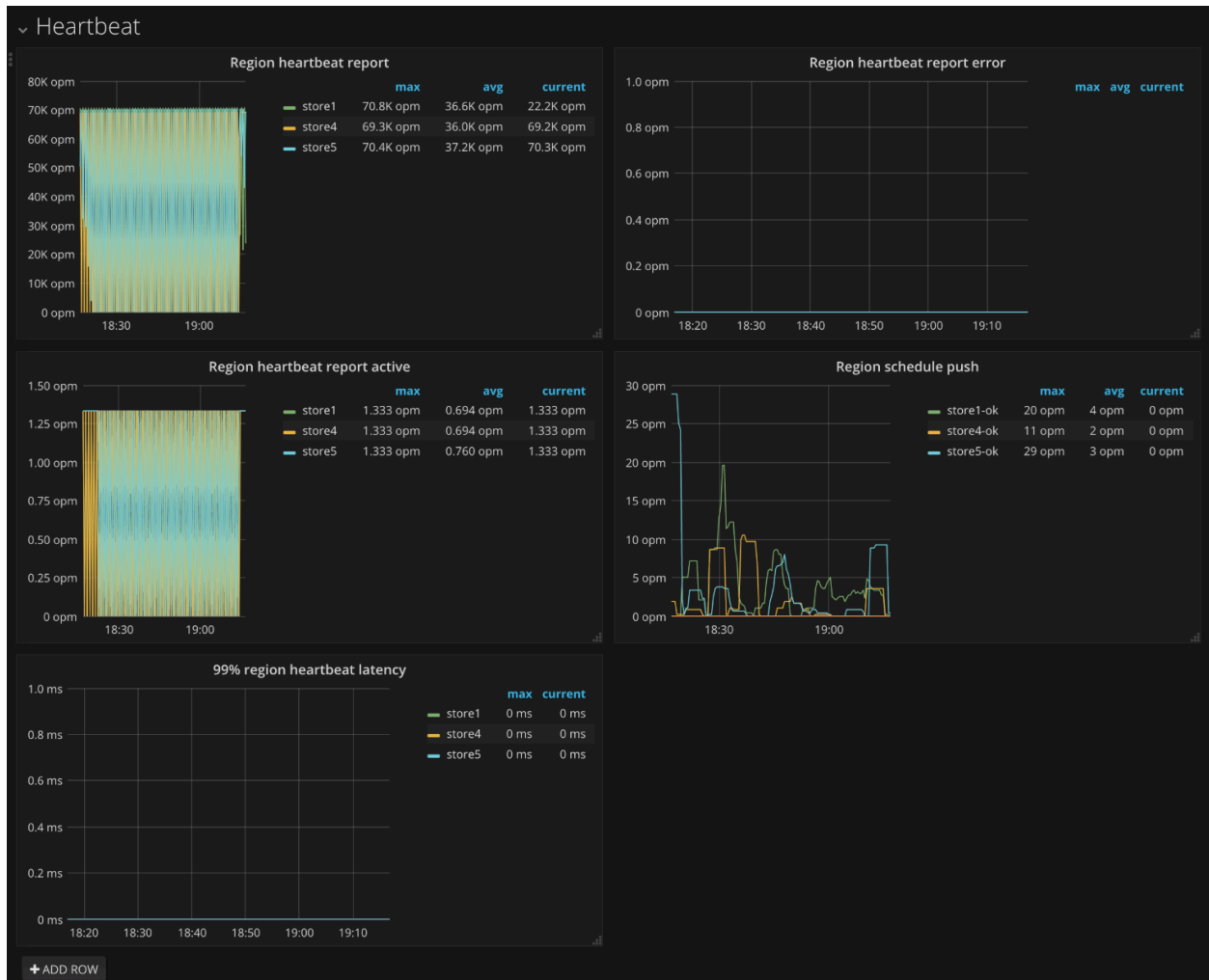
图 230: PD Dashboard - Heartbeat metrics
