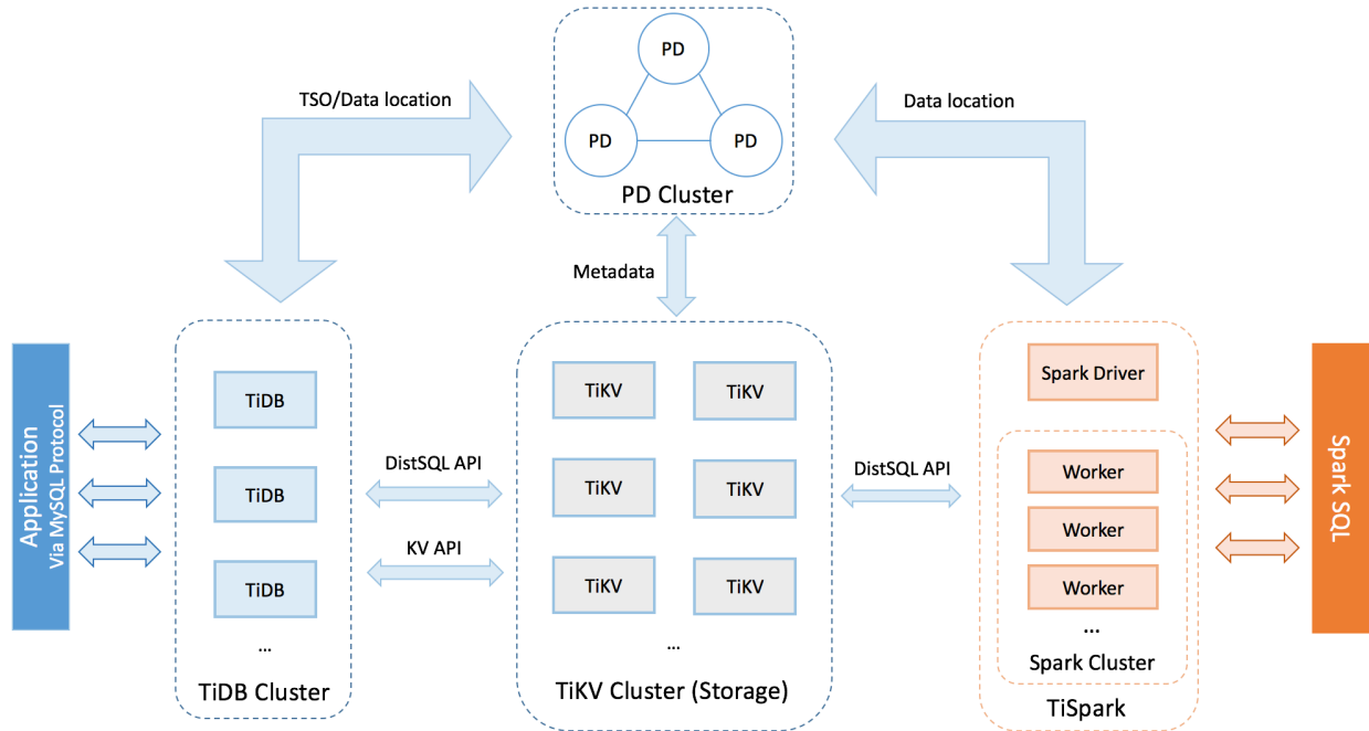
图 8: TiDB Architecture
