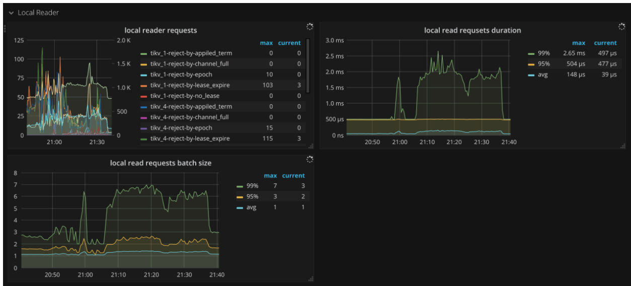
图 239: TiKV Dashboard - Local reader metrics
