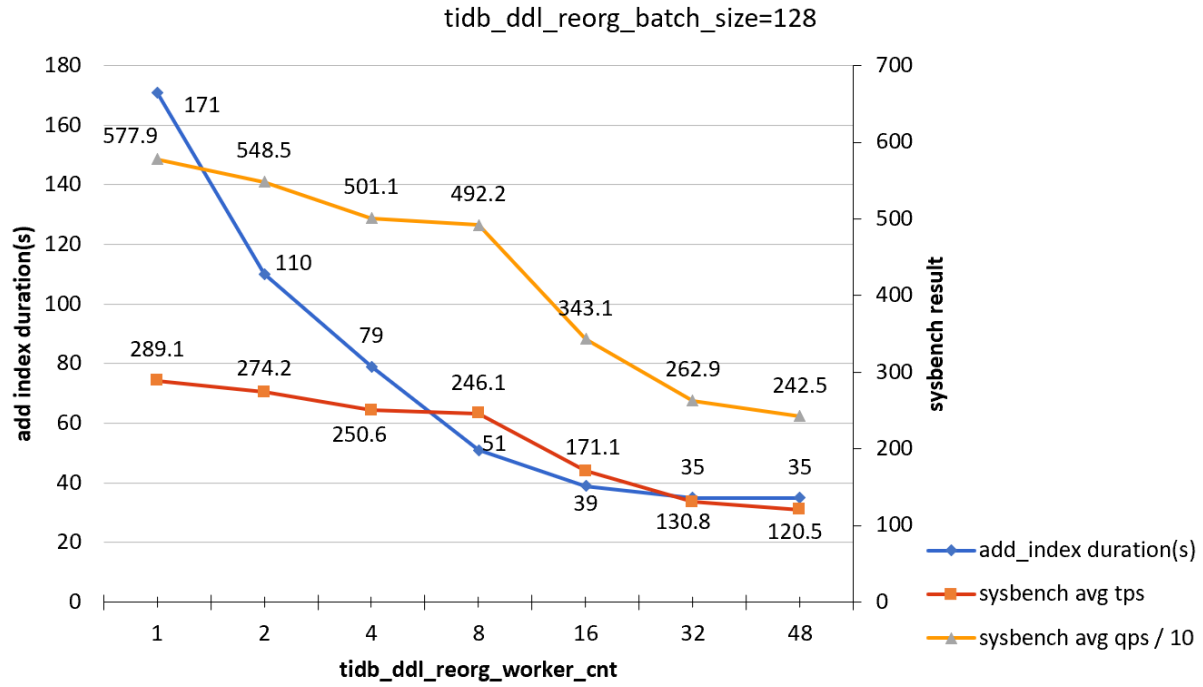
图 11: add-index-load-1-b128
