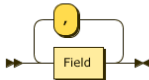
图 189: SelectStmtFieldList
