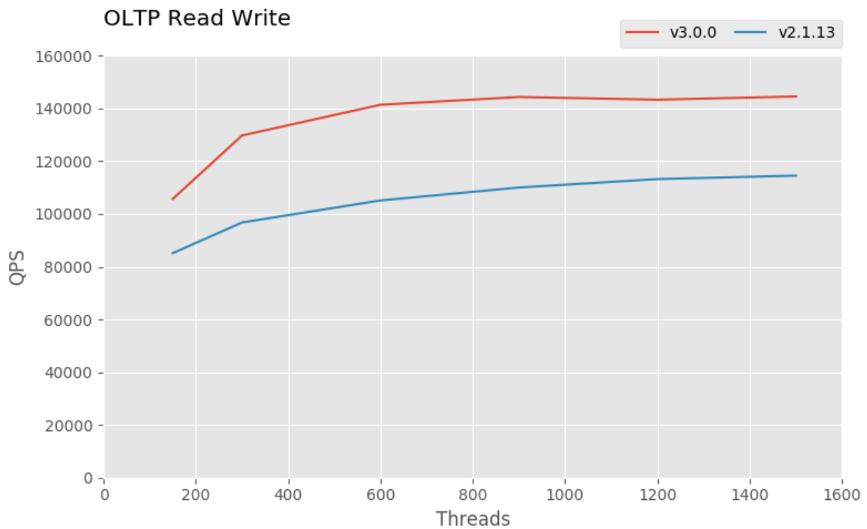
图 7: read write
