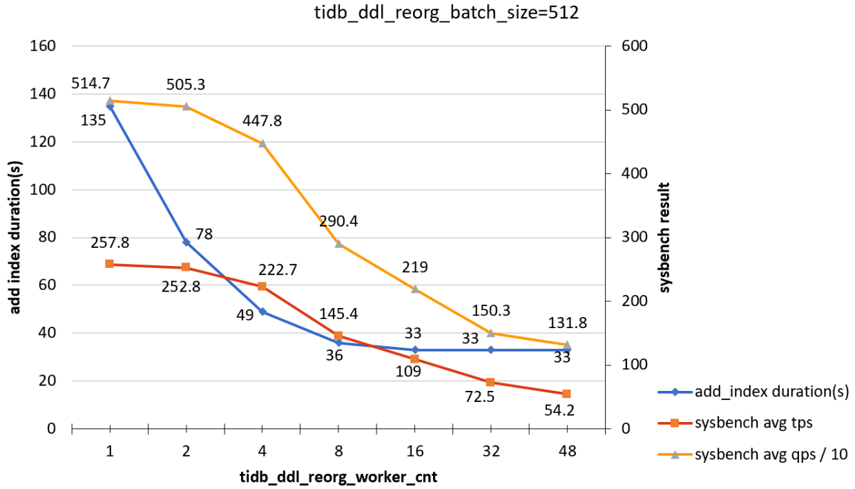
图 13: add-index-load-1-b512
