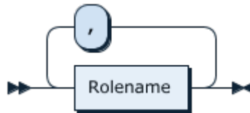
图 182: RolenameList
