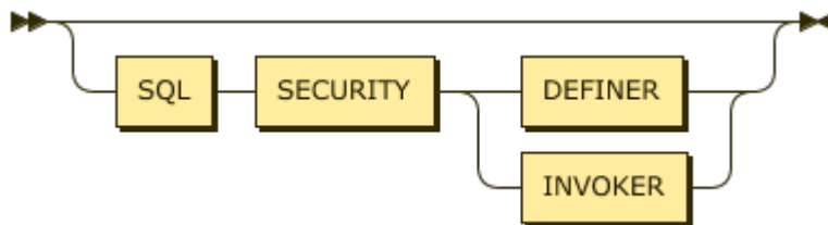
图 86: ViewSQLSecurity
