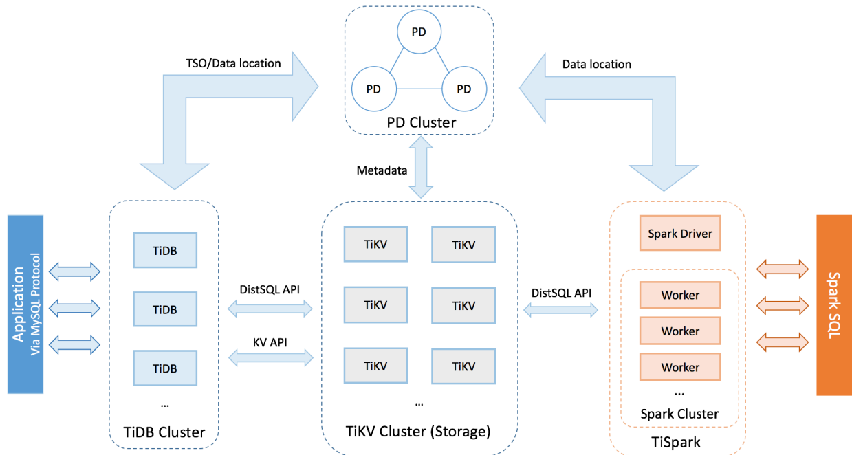
图 23: TiDB Architecture
