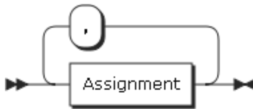
图 263: AssignmentList
