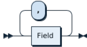
图 216: SelectStmtFieldList
