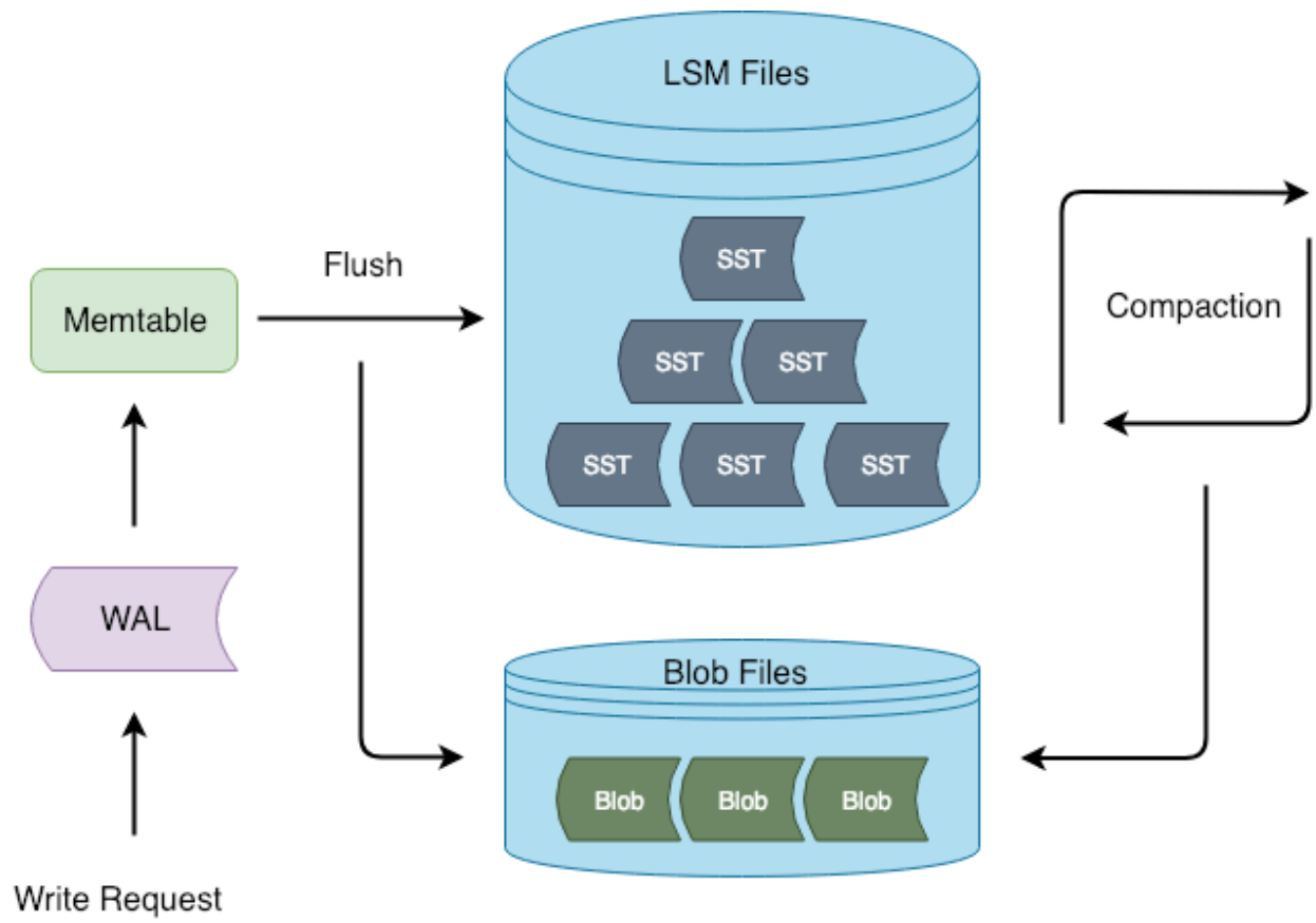
图 180: Architecture
