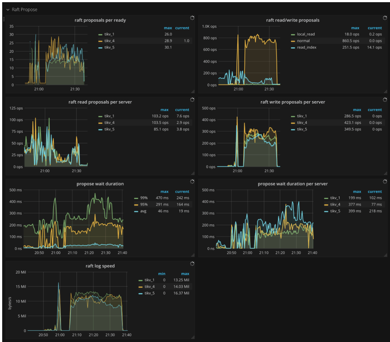
图 207: TiKV Dashboard - Raft propose metrics
