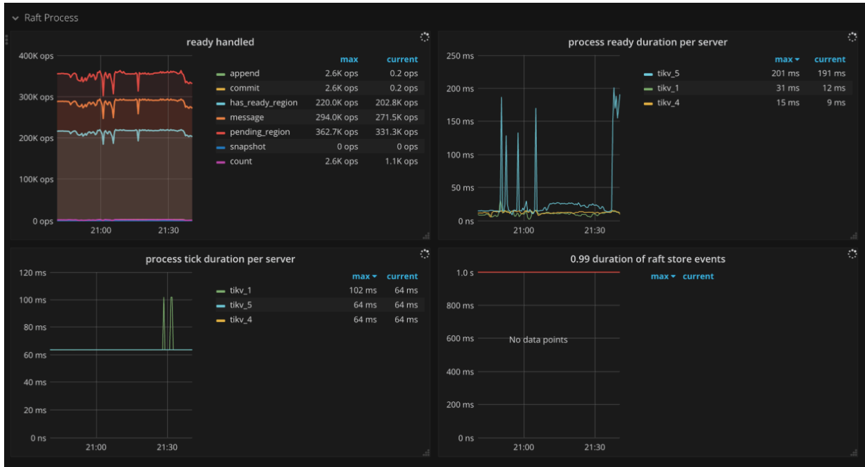
图 205: TiKV Dashboard - Raft process metrics
