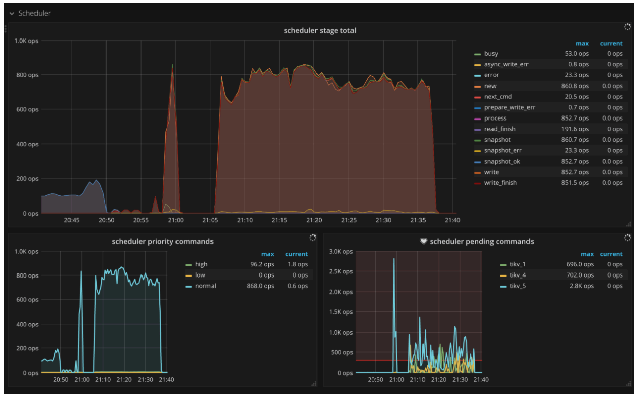
图 211: TiKV Dashboard - Scheduler metrics
