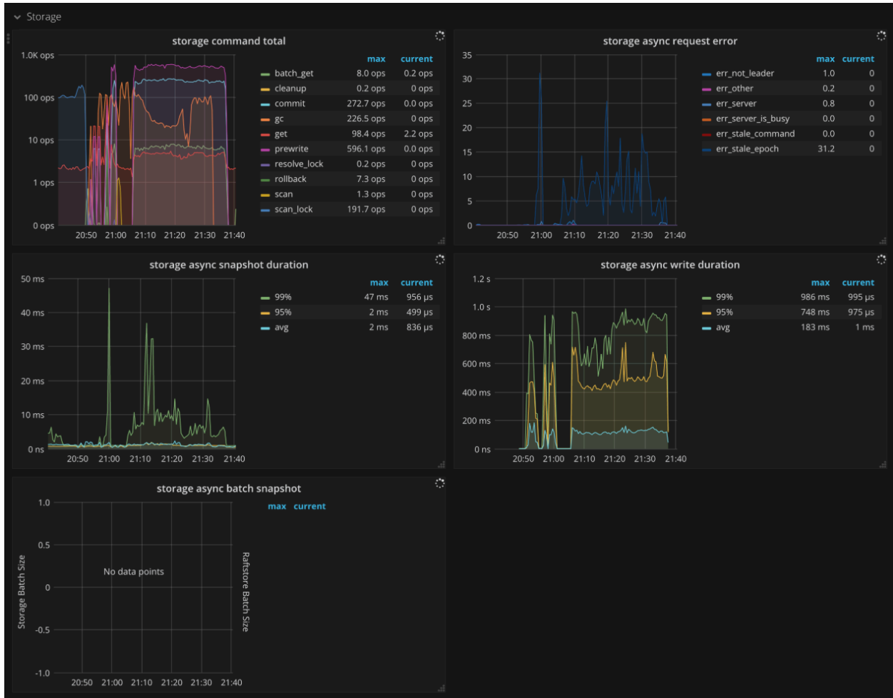
图 210: TiKV Dashboard - Storage metrics
