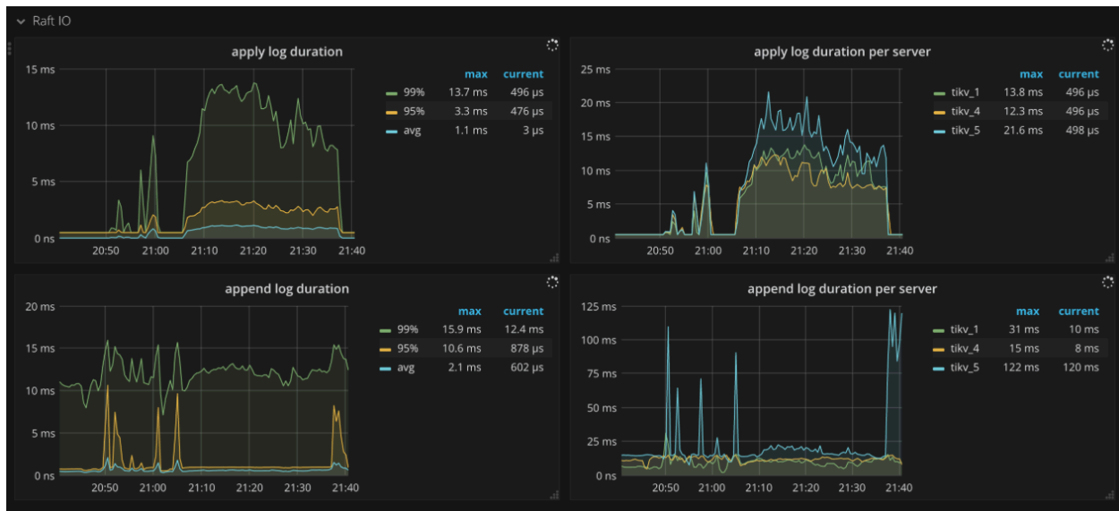
图 204: TiKV Dashboard - Raft IO metrics
