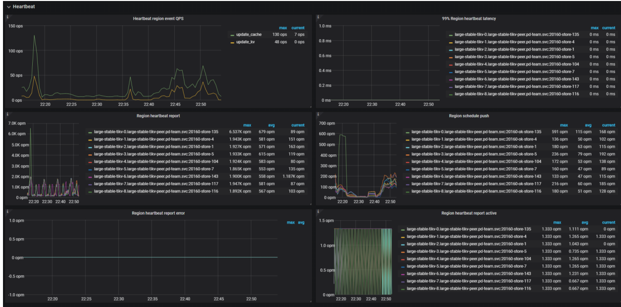
图 199: PD Dashboard - Heartbeat metrics
