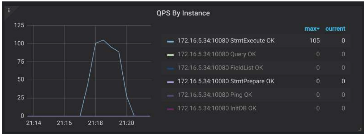
图 83: QPS By Instance
