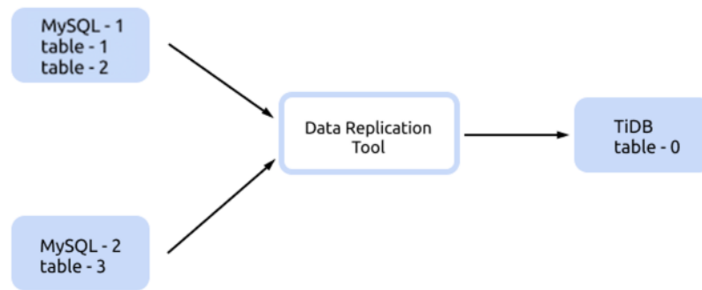
Figure 304: shard-table-replica-1
