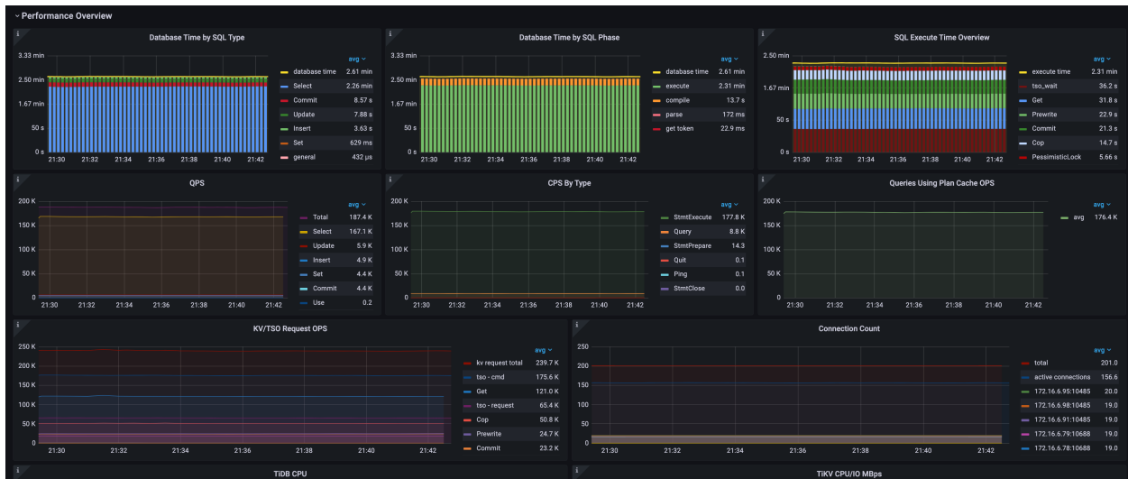
Figure 587: performance overview
