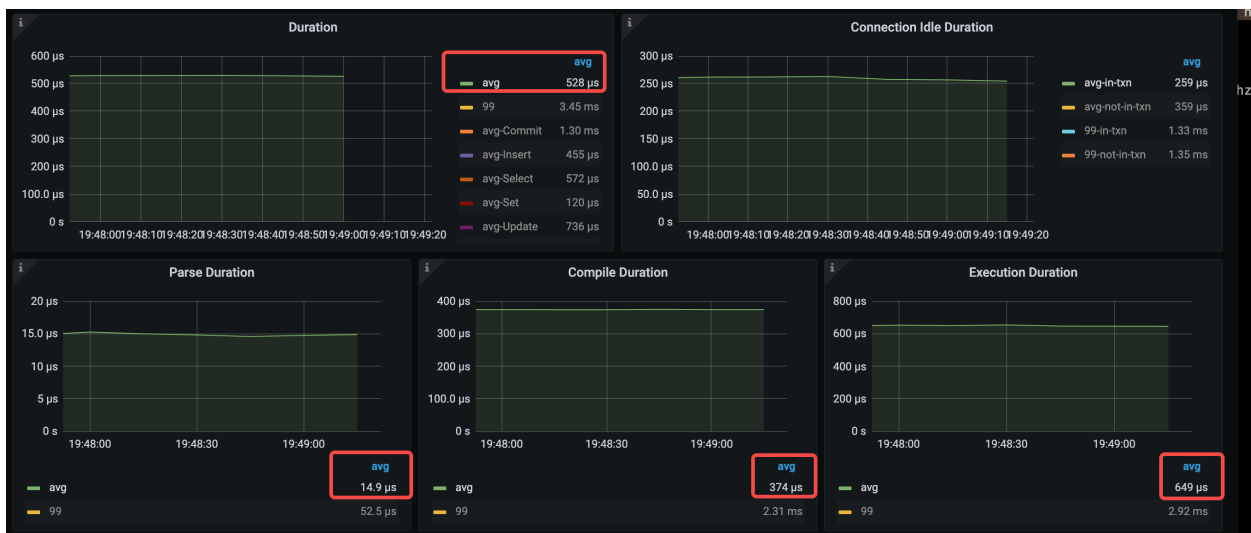
Figure 151: performance-overview-2-for-PrepStmts
