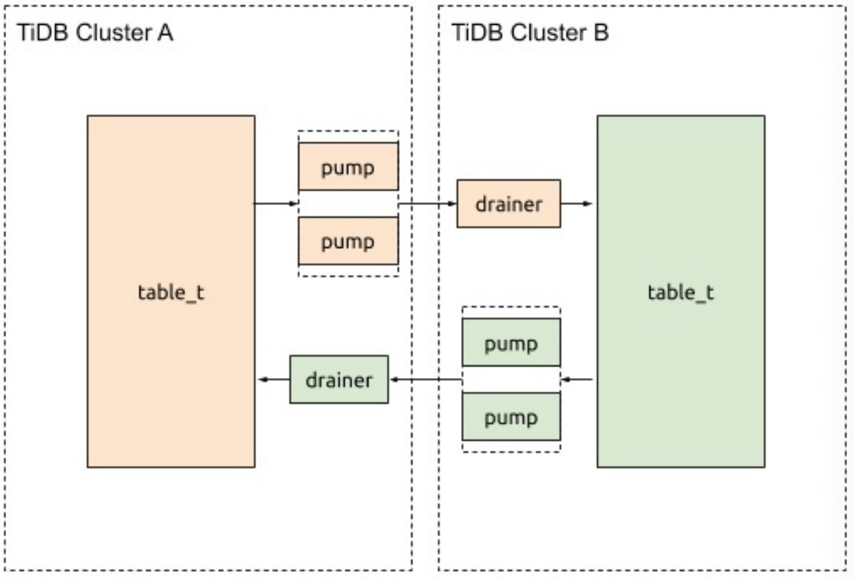
Figure 294: Architect
