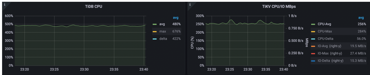
Figure 167: performance-overview-2-for-table-cache
