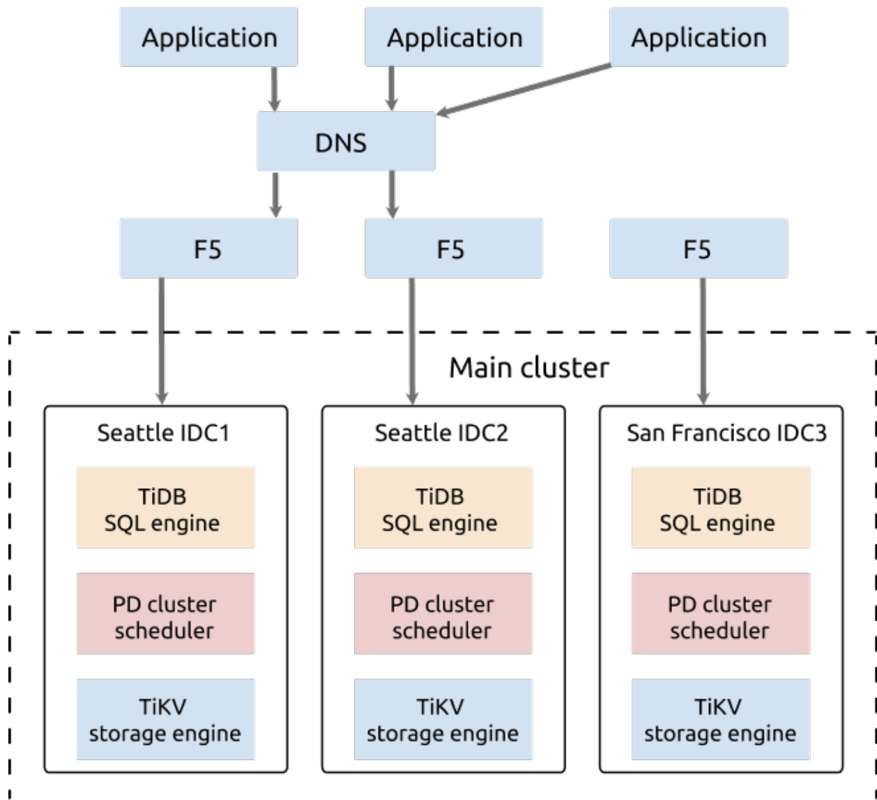
Figure 185: 3-DC-in-2-city architecture
