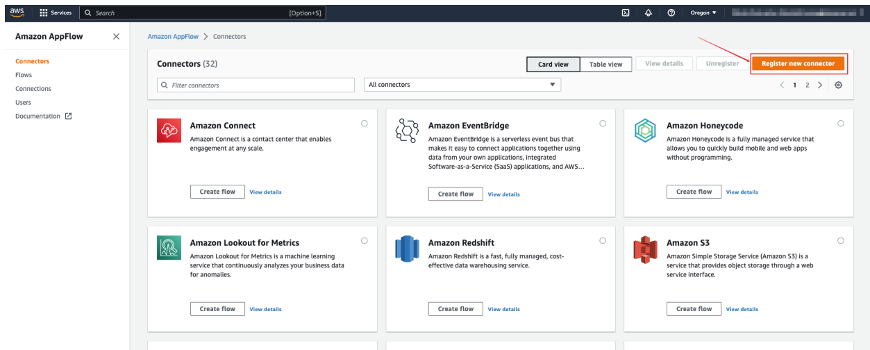
Figure 23: register connector
