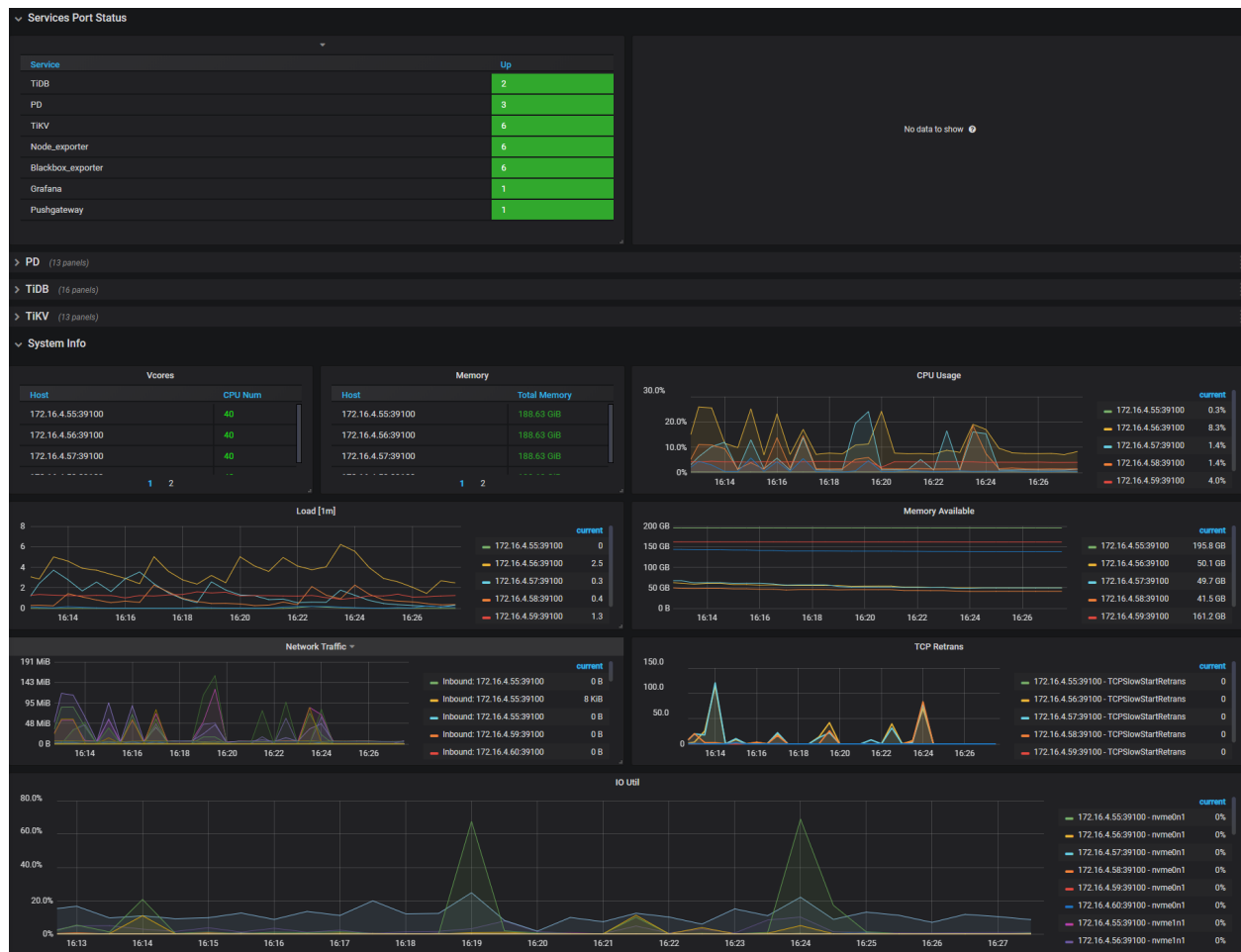
Figure 326: overview
