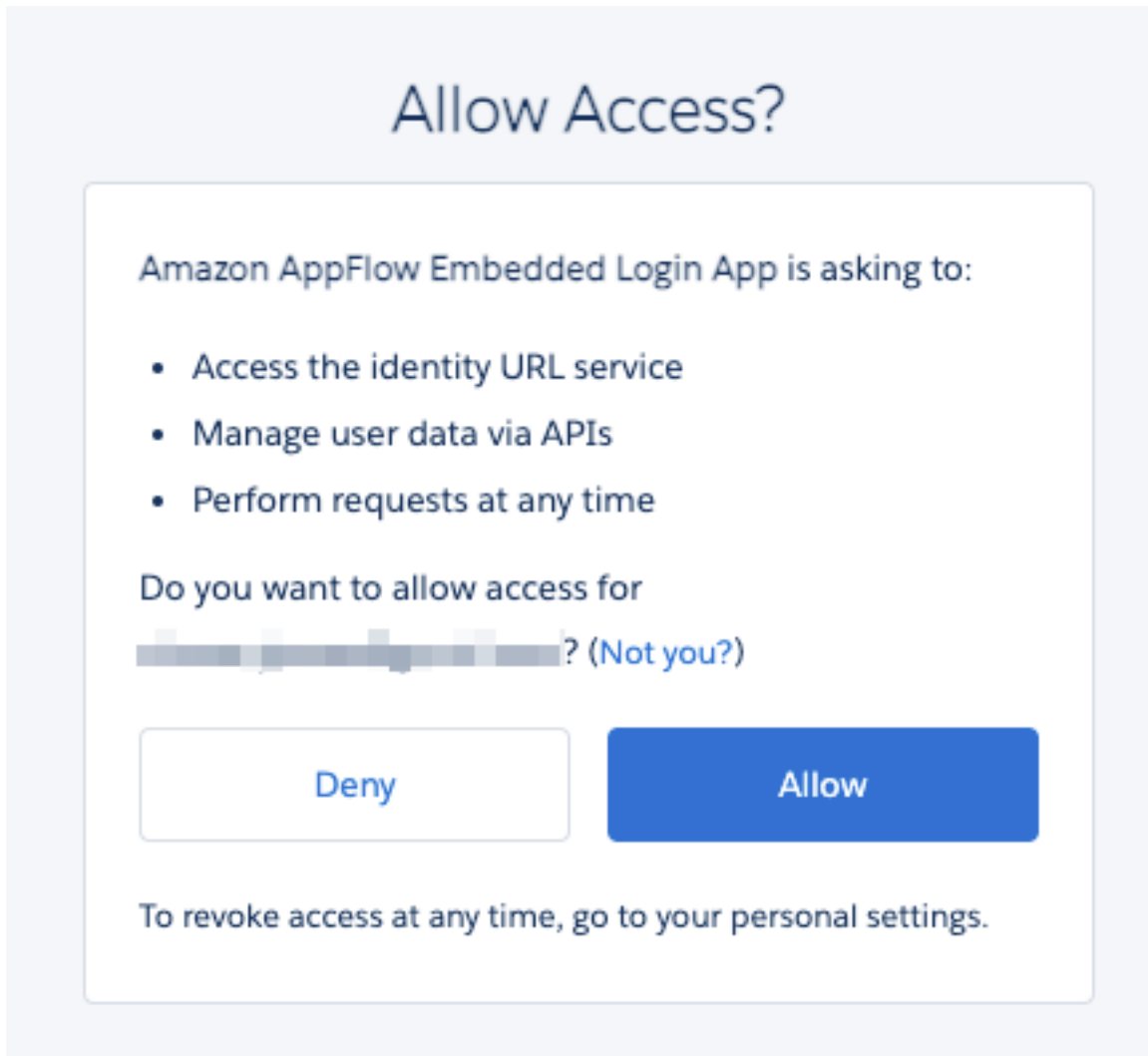
Figure 30: allow salesforce
