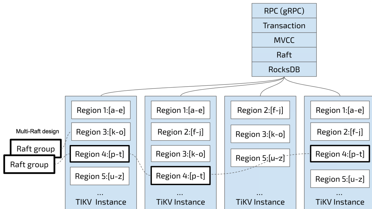
Figure 311: TiDB Storage
