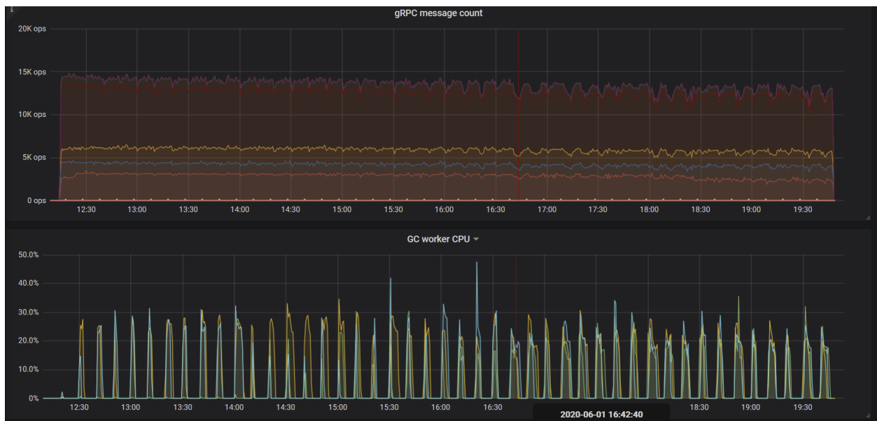
Figure 226: GC Impact
