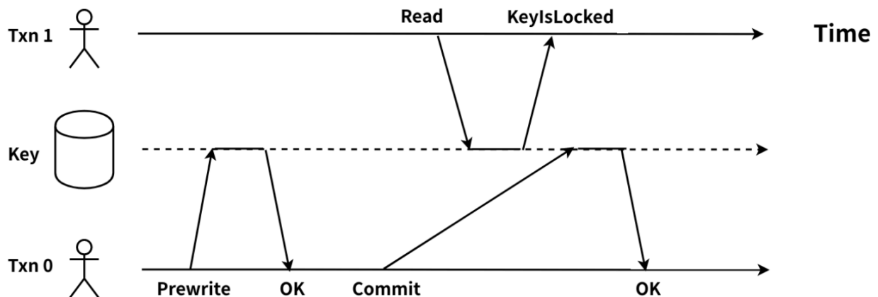
Figure 106: read-write conflict
