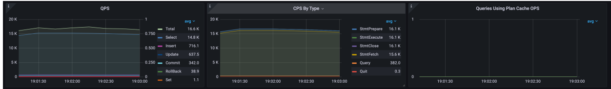
Figure 118: OLTP-Prepared
