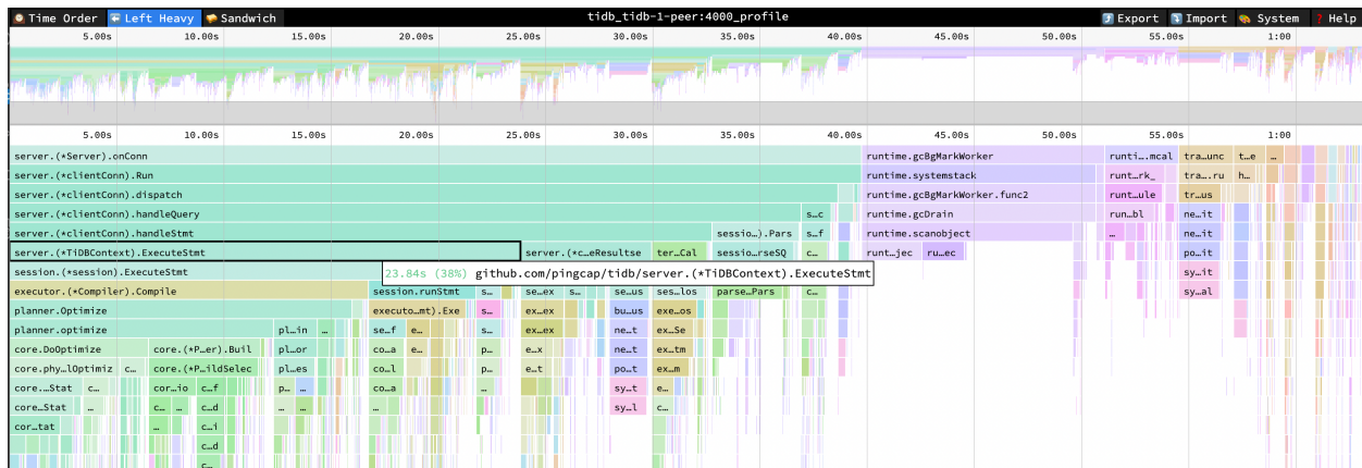
Figure 140: flame-graph-for-query-interface
