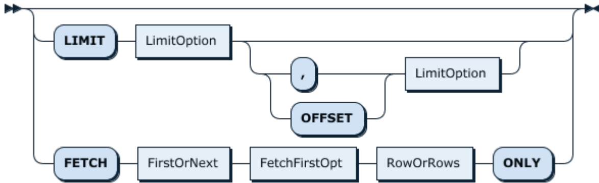
Figure 367: SelectStmtLimit
