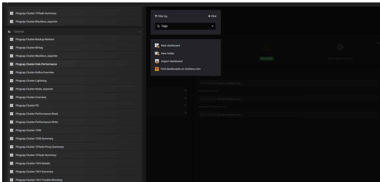
Figure 87: Grafana monitored_groups
