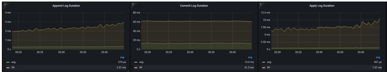
Figure 135: v5.3.0
