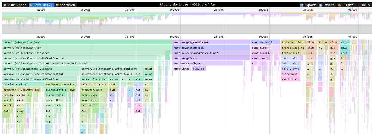
Figure 160: flame-graph-for-rc-read
