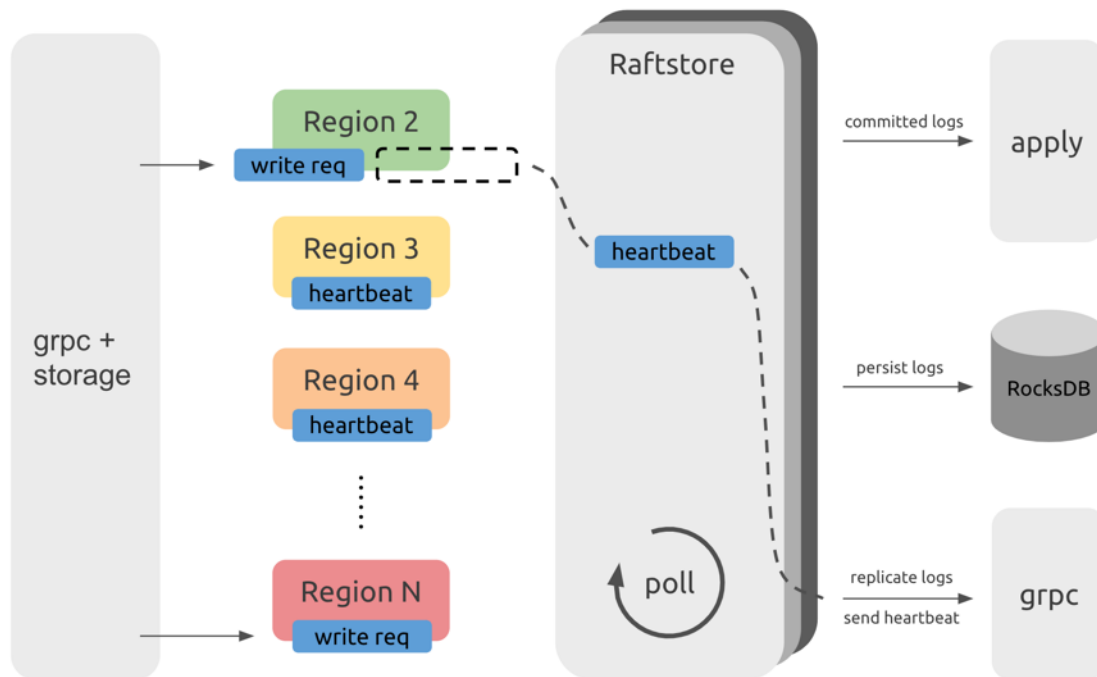
Figure 218: Raftstore Workflow
