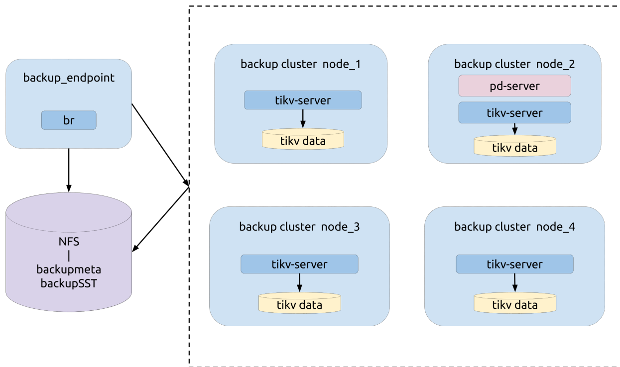
Figure 57: img
