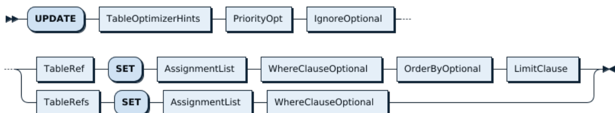
Figure 480: UpdateStmt
