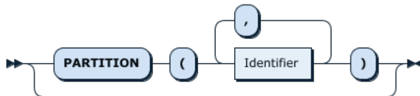
Figure 469: PartitionNameListOpt
