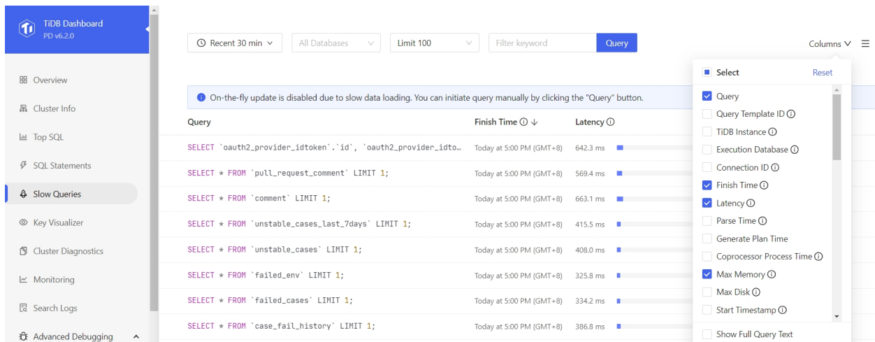
Figure 552: Show more columns
