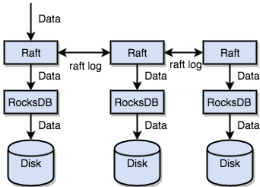
Figure 309: Raft in TiDB
