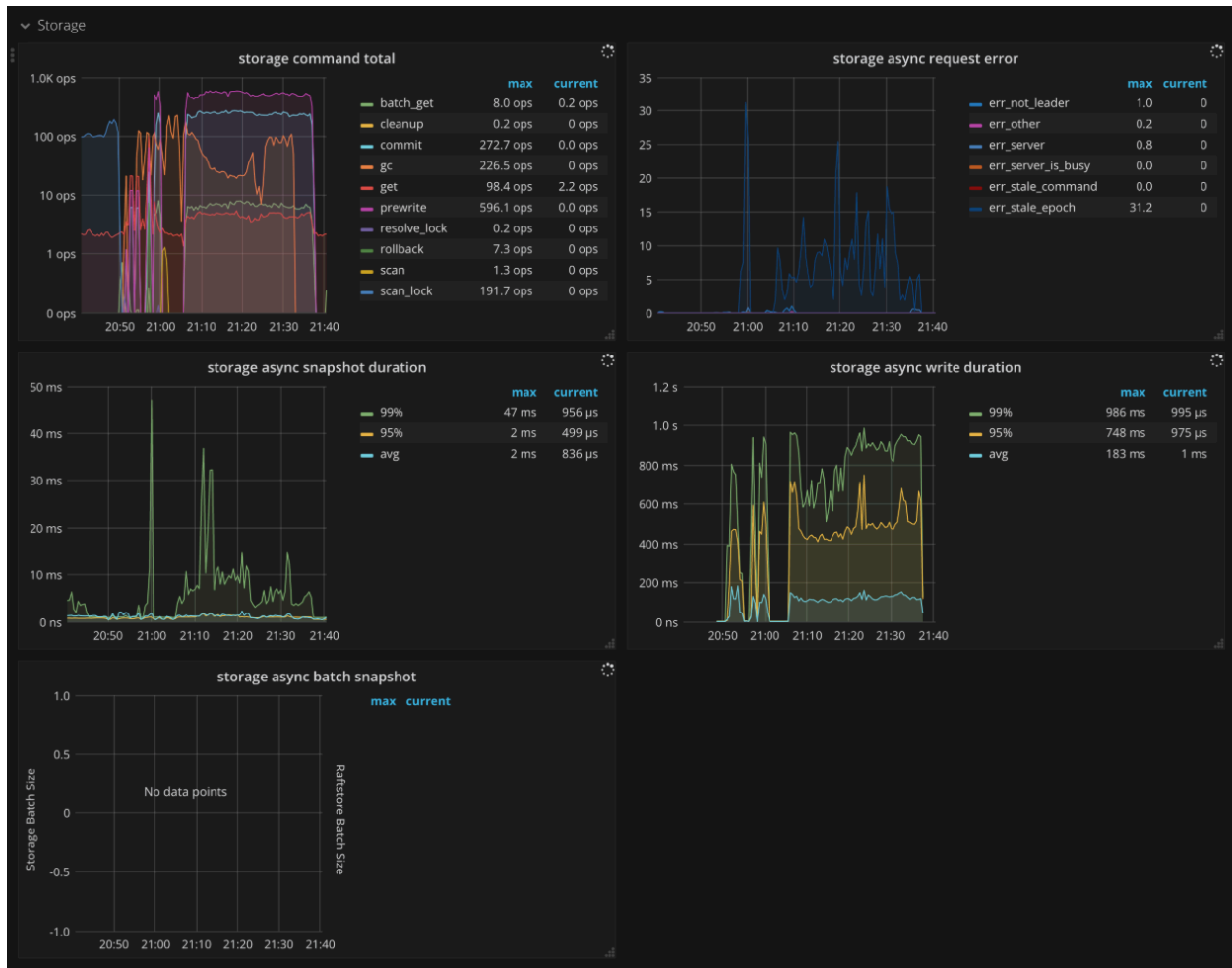
Figure 348: TiKV Dashboard - Storage metrics
