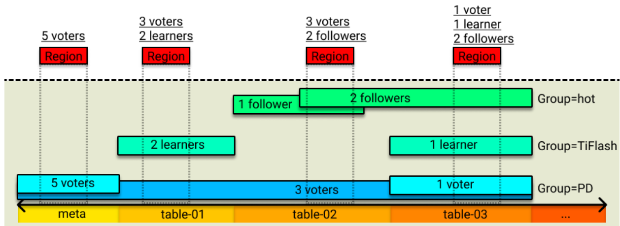
Figure 227: Placement rules overview
