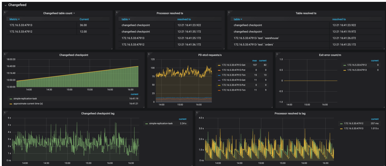
Figure 300: TiCDC Dashboard - Changefeed metrics 1
