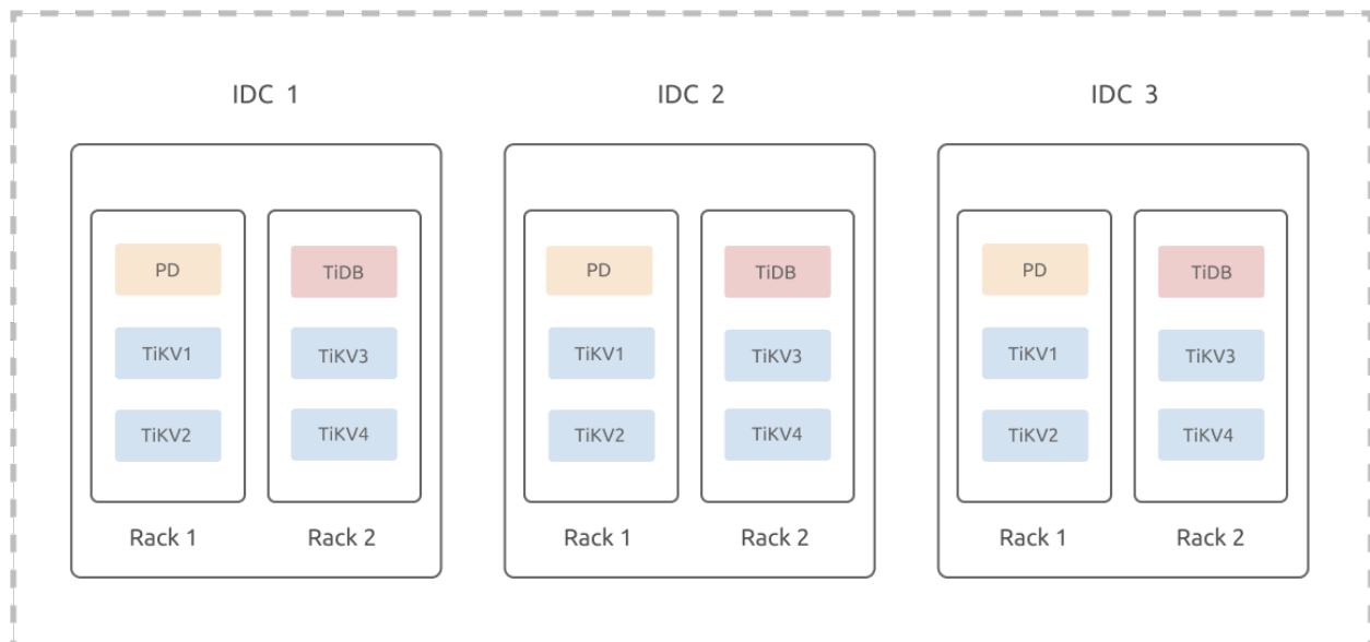
Figure 184: 3-DC in One City
