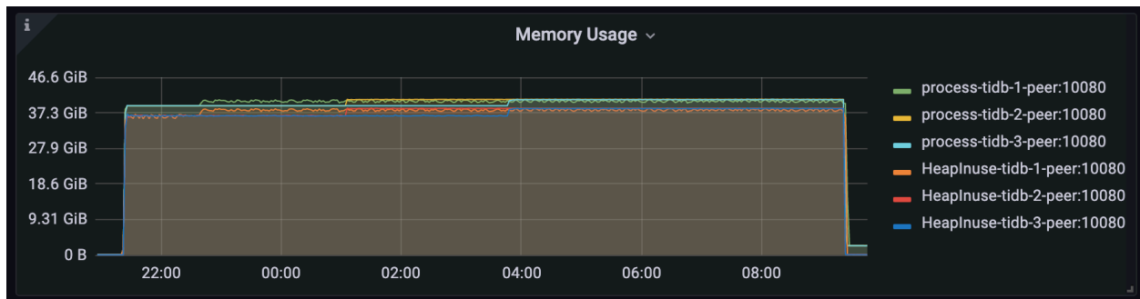
Figure 171: v6.1.3 workload no oom with GOMEMLIMIT
