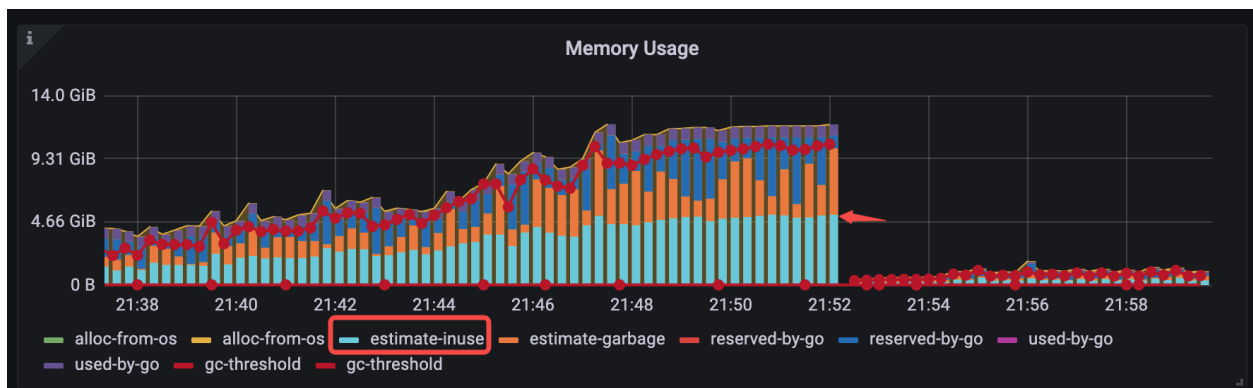
Figure 169: normal OOM case example
