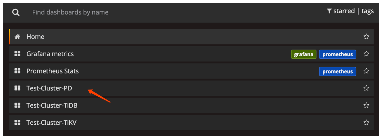
Figure 89: view dashboard
