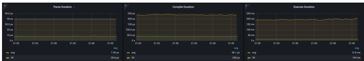
Figure 126: Execute
