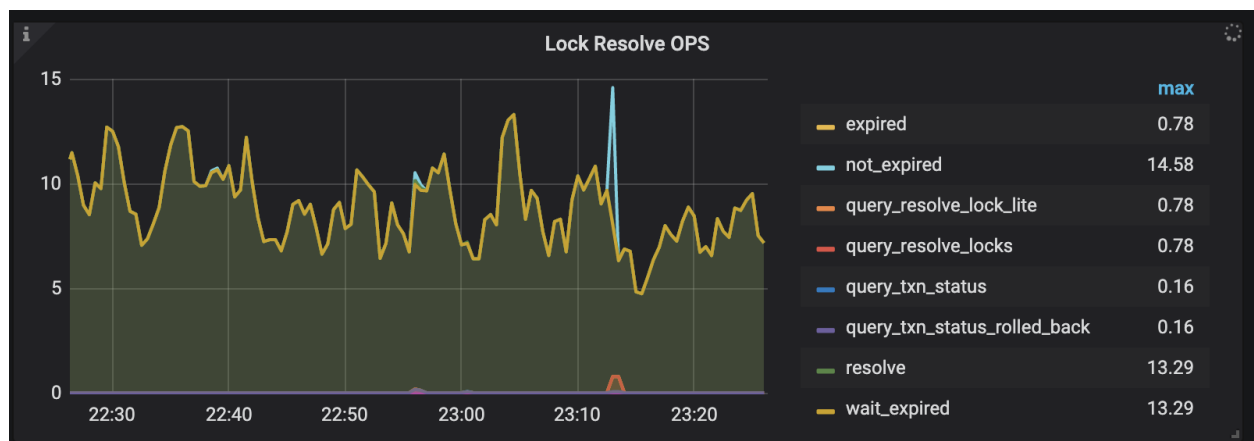
Figure 108: lock-resolve-ops
