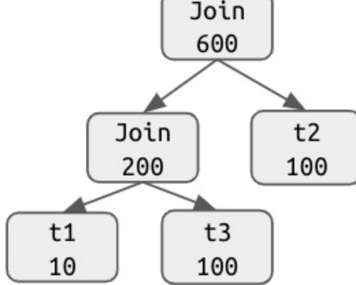
Figure 175: join-reorder-3
