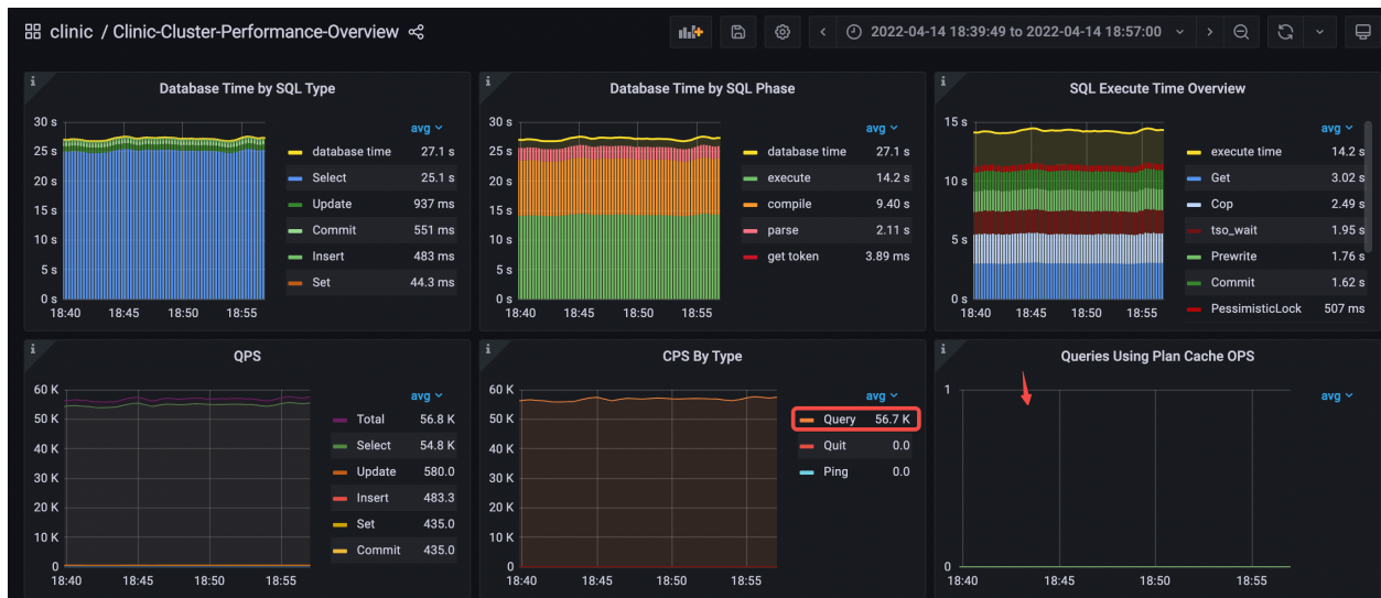
Figure 141: performance-overview-1-for-query-interface
