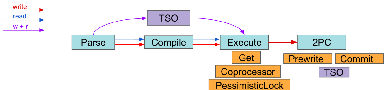
Figure 127: Execute
