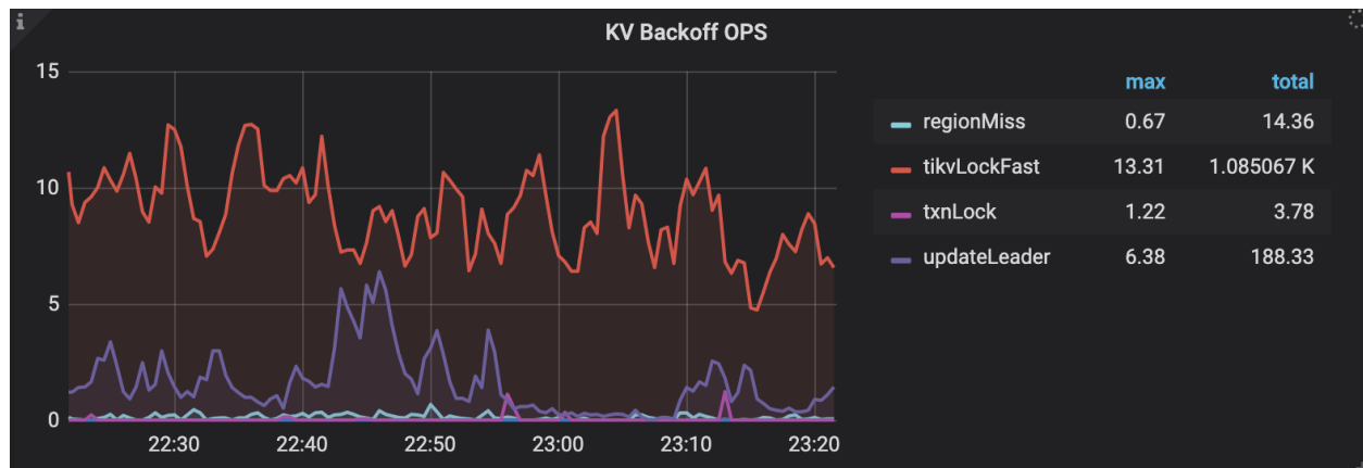
Figure 107: kv-backoff-ops
