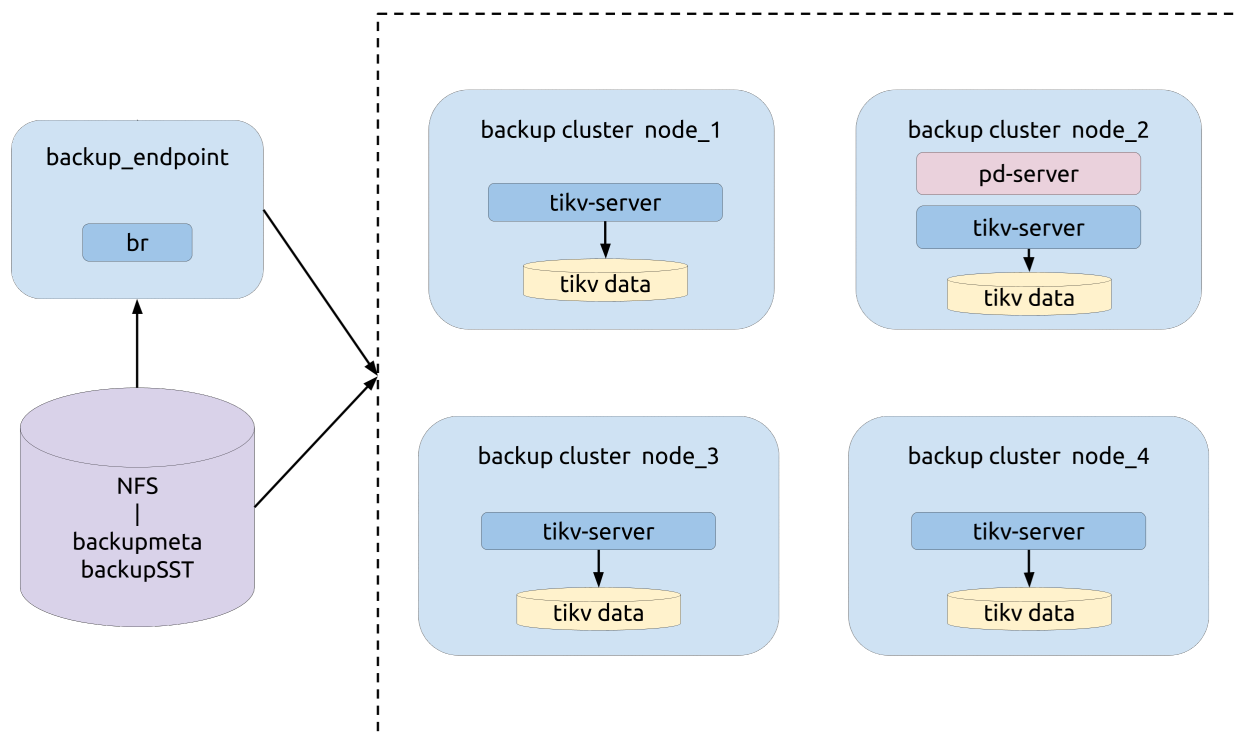
Figure 278: img
