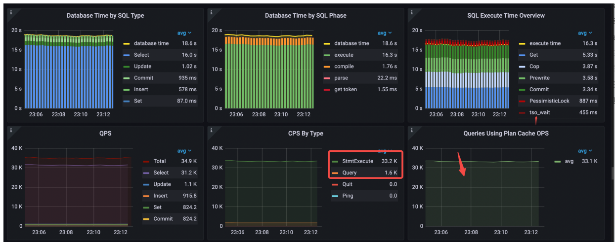
Figure 161: performance-overview-1-for-rc-read
