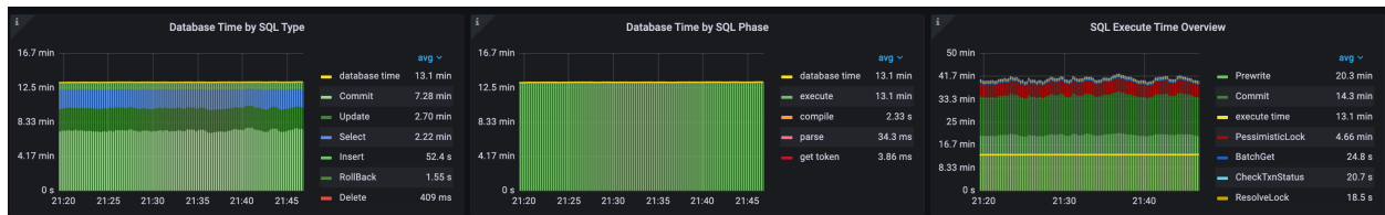
Figure 112: TPC-C
