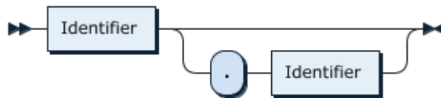
Figure 412: TableName
