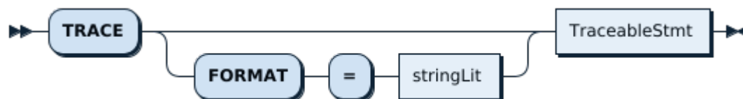
Figure 473: TraceStmt
