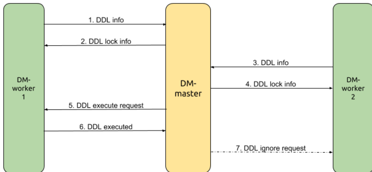
Figure 247: shard-ddl-flow
