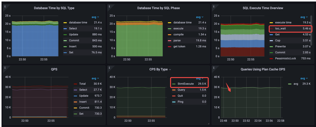
Figure 157: performance-overview-for-1-command
