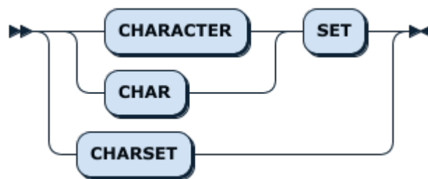
Figure 395: CharsetKw
