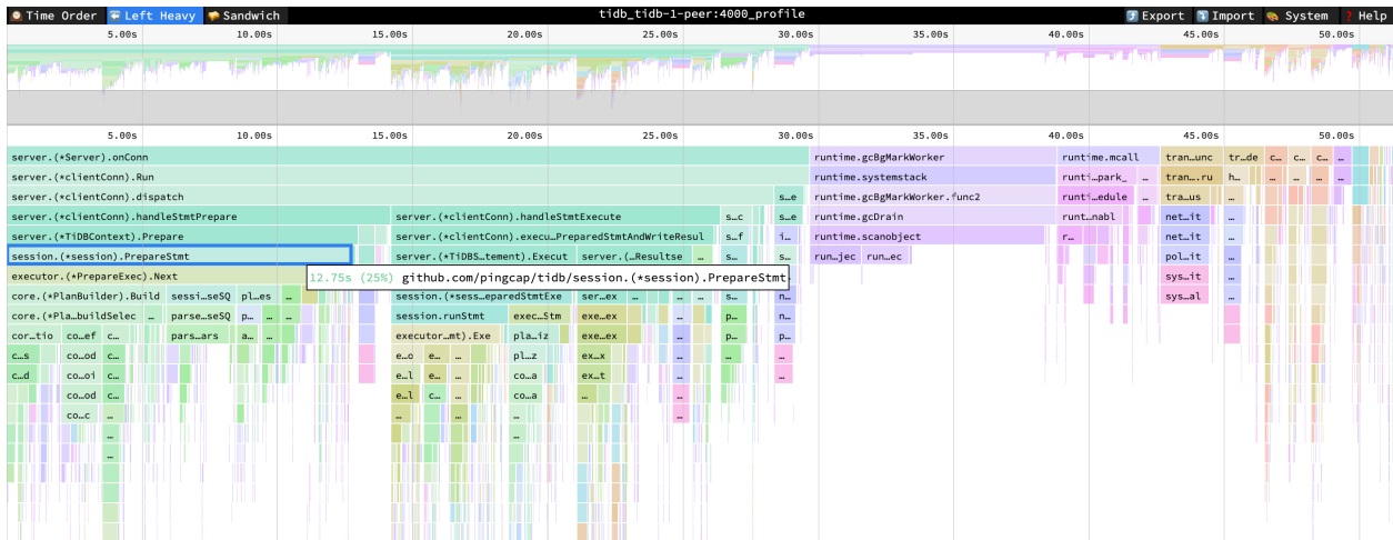
Figure 152: flame-graph-for-3-commands
