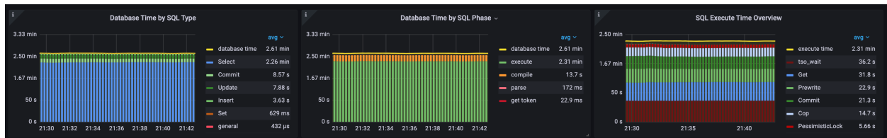
Figure 113: OLTP
