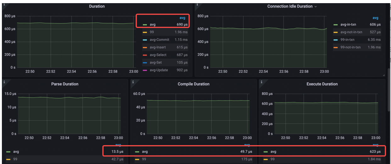
Figure 159: performance-overview-for-3-command
