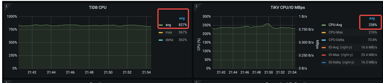
Figure 154: performance-overview-2-for-3-commands
