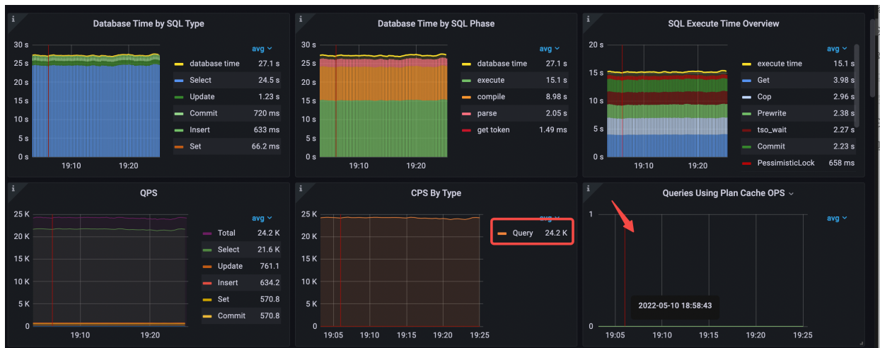
Figure 145: performance-overview-1-for-maxPerformance
