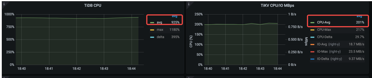
Figure 142: performance-overview-2-for-query-interface
