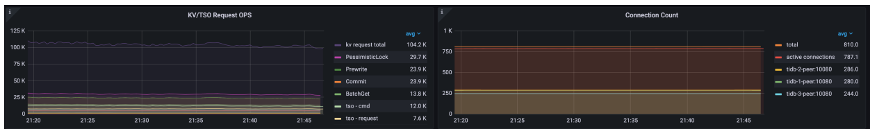
Figure 119: TPC-C
