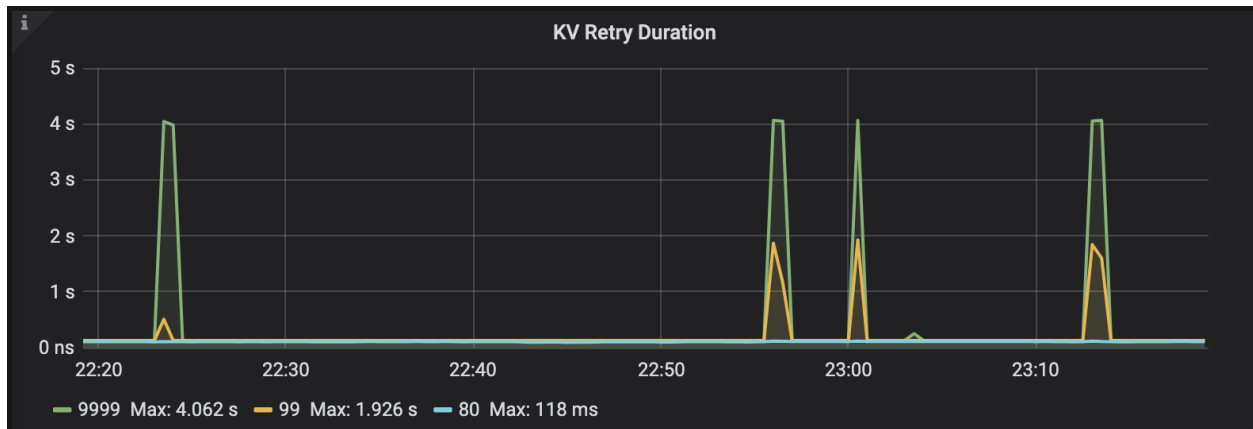
Figure 109: kv-retry-duration
