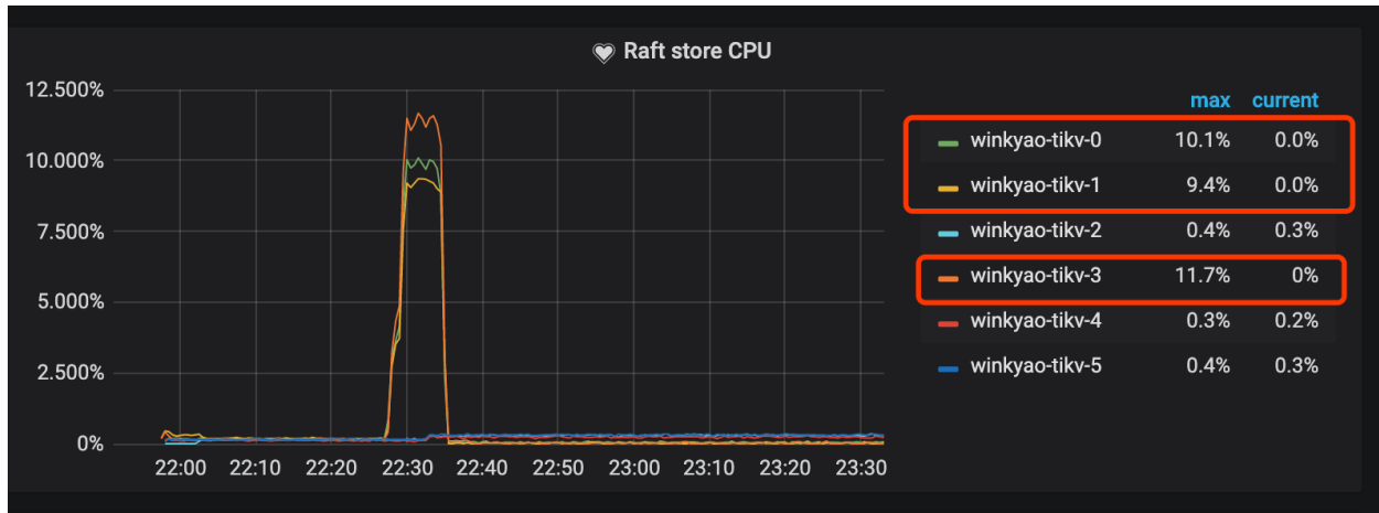
Figure 194: QPS3
