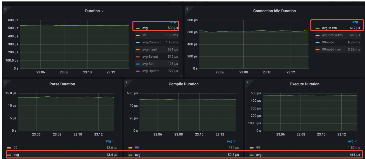
Figure 164: performance-overview-4-for-rc-read
