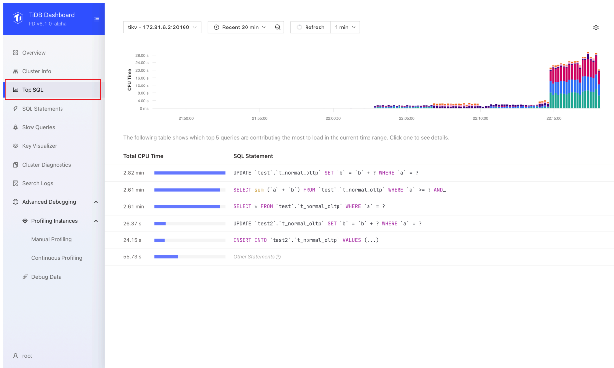
Figure 92: Top SQL
