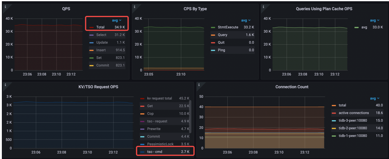
Figure 162: performance-overview-2-for-rc-read
