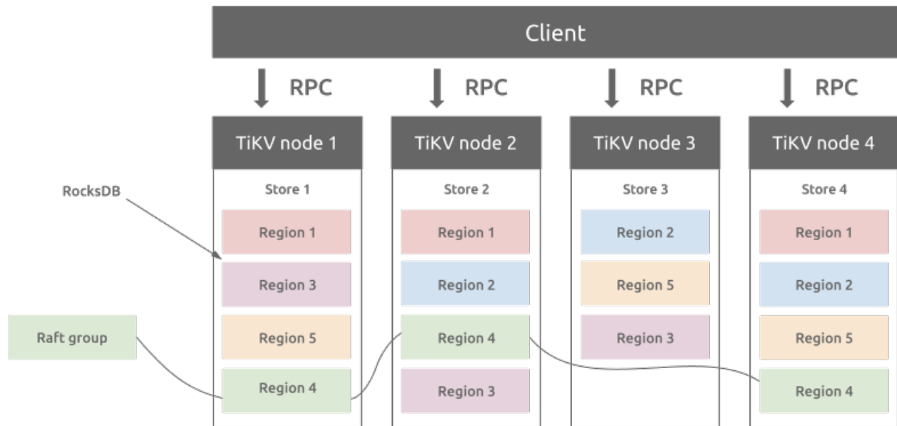
Figure 316: TiKV Architecture
