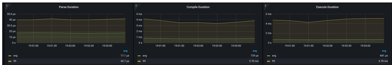
Figure 125: Compile
