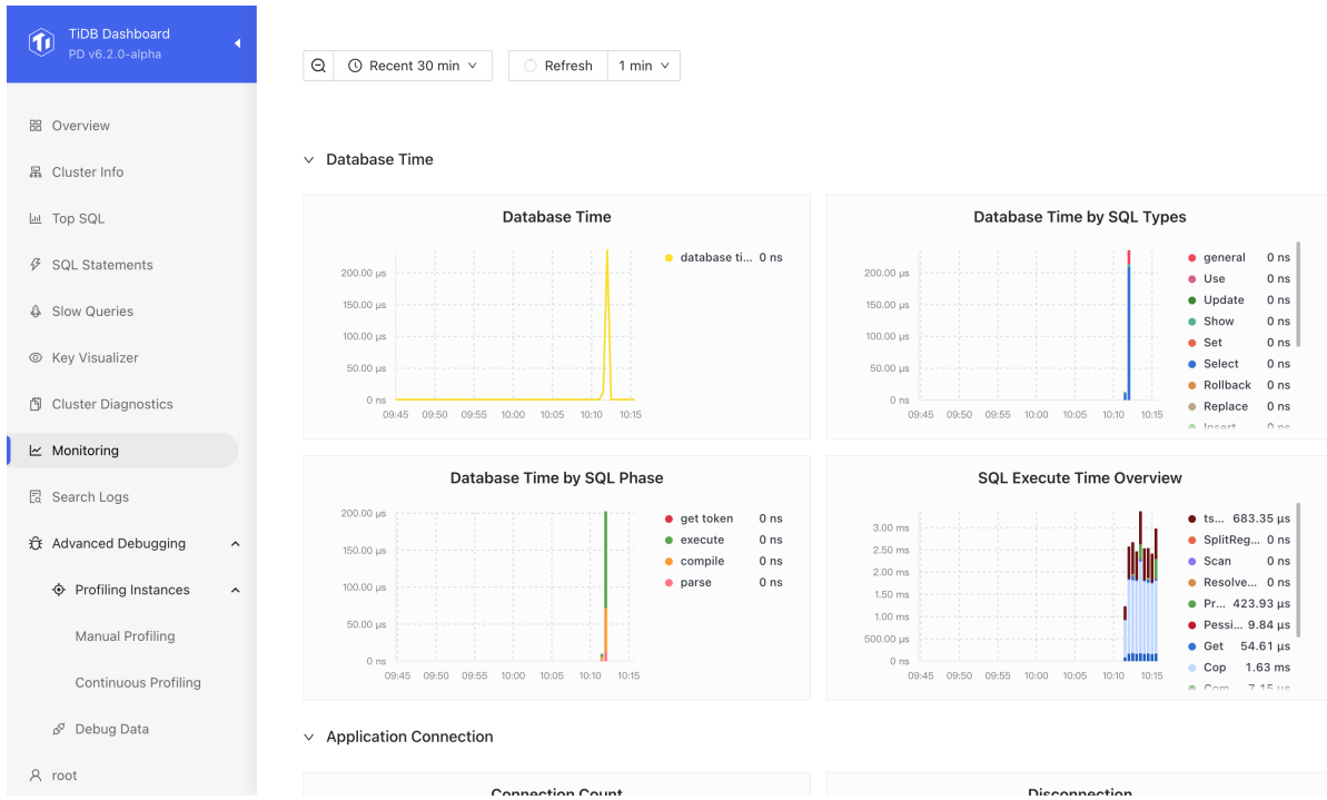
Figure 586: Monitoring page
