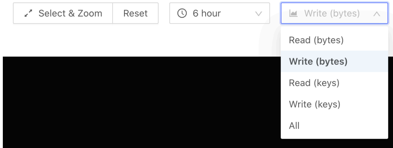
Figure 523: Select metrics
