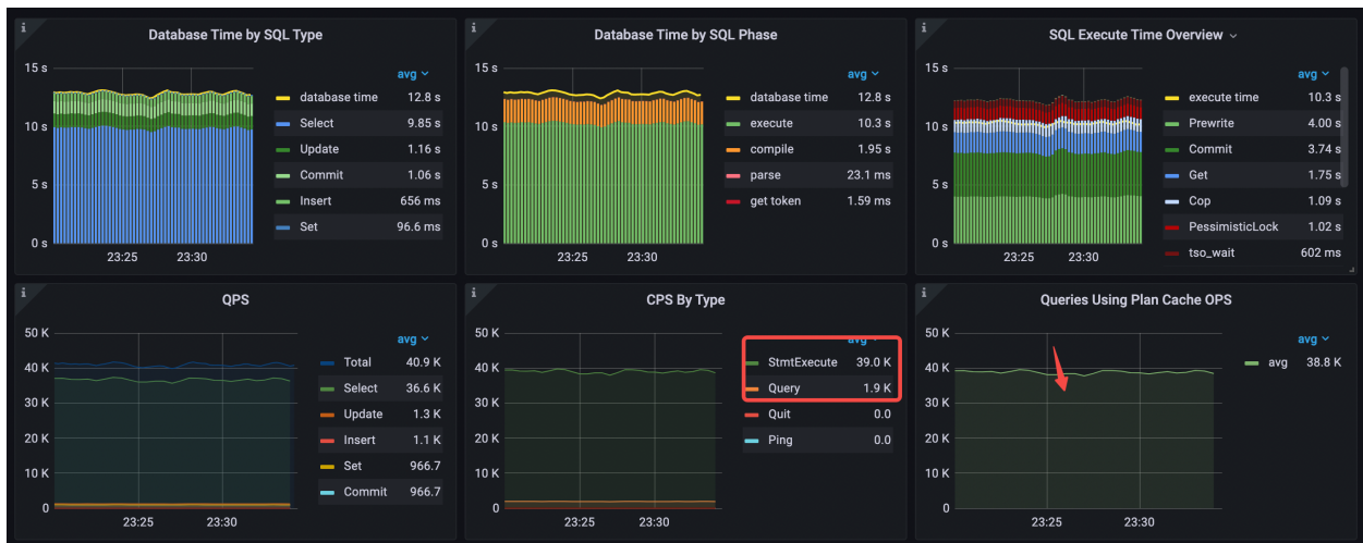
Figure 166: performance-overview-1-for-table-cache
