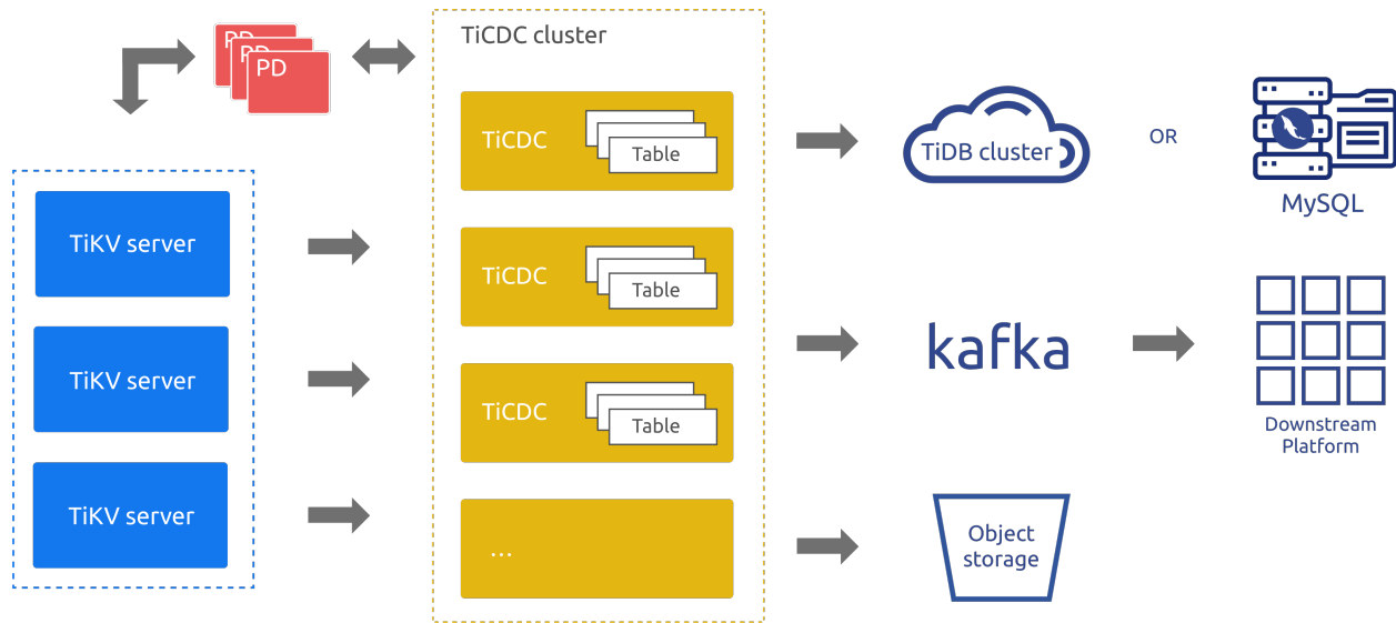
图 39: TiCDC architecture
