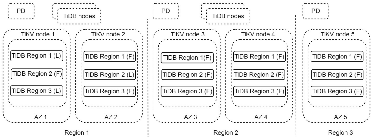
图 42: Multi-replica cluster DR
