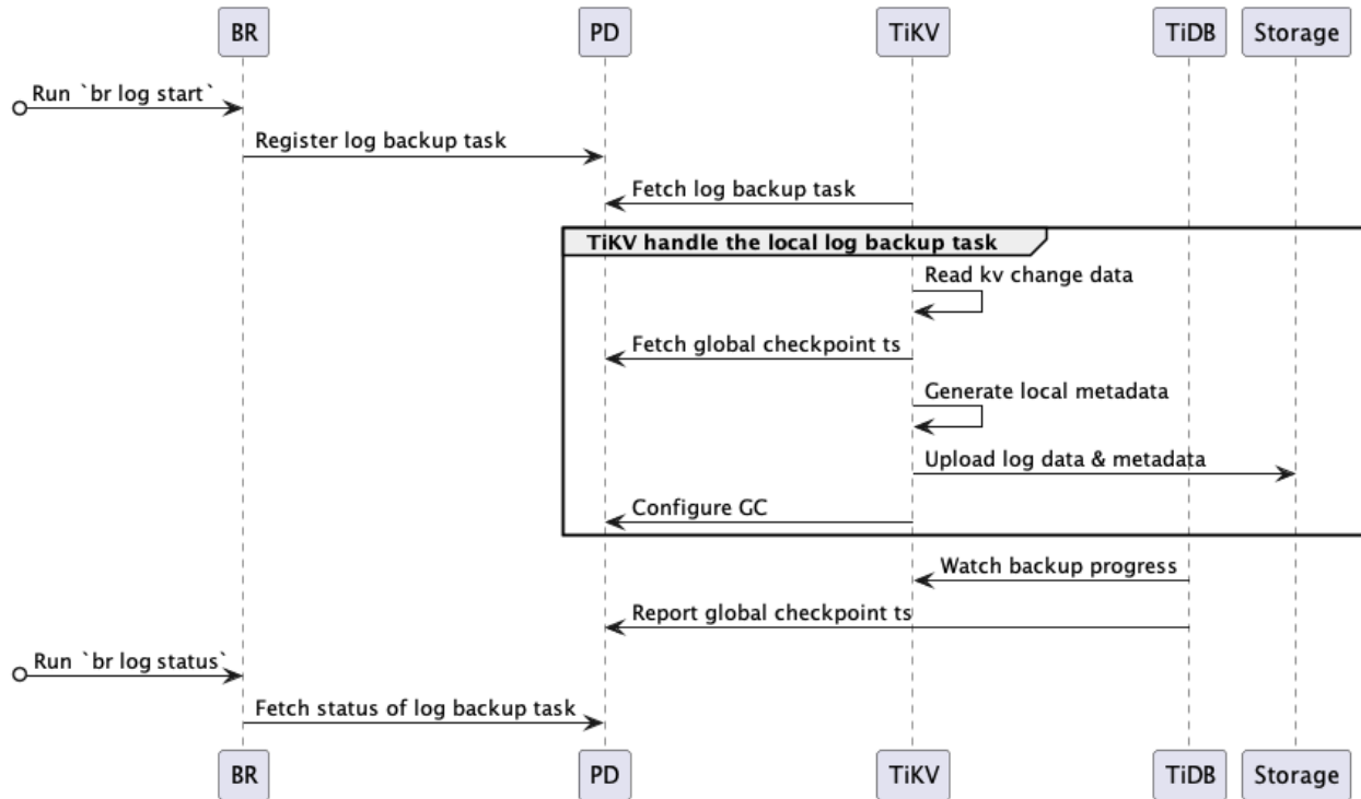
图 34: BR log backup process design
