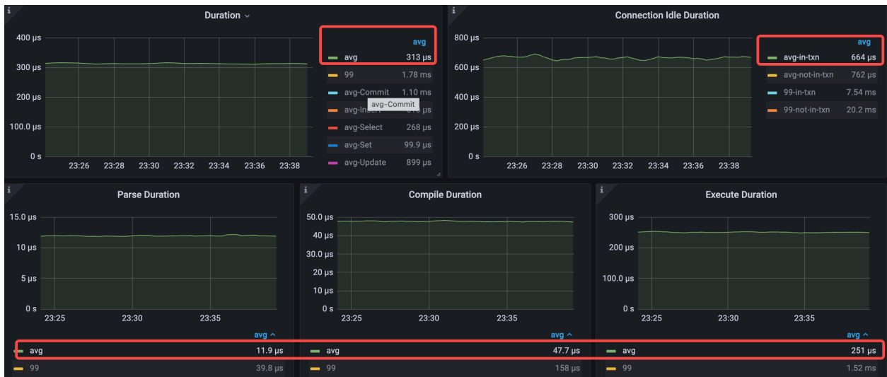
图 142: performance-overview-3-for-table-cache
