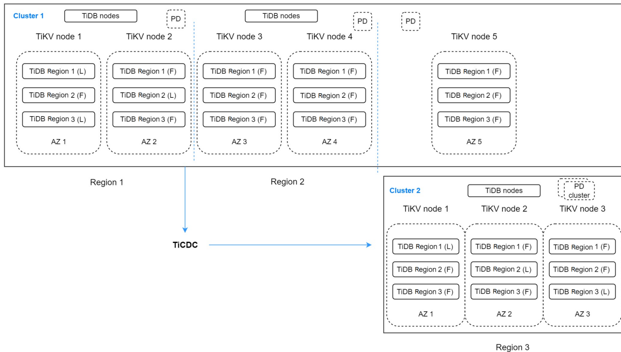
图 43: TiCDC-based multi-replica cluster DR
