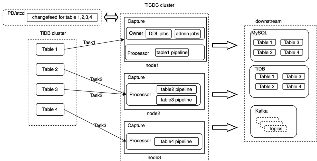
图 277: TiCDC architecture
