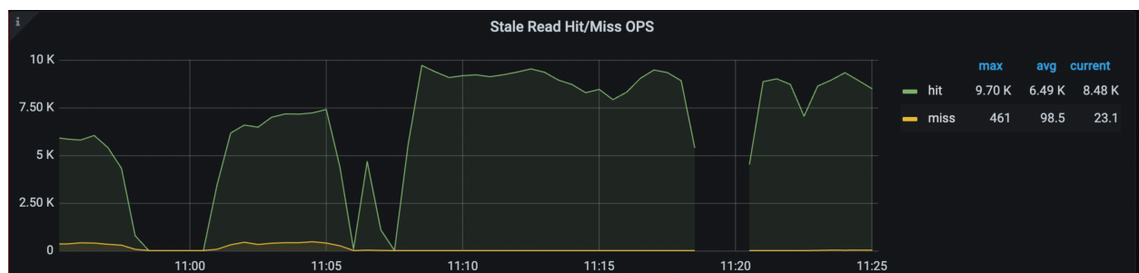
图 98: Stale Read Hit/Miss OPS
