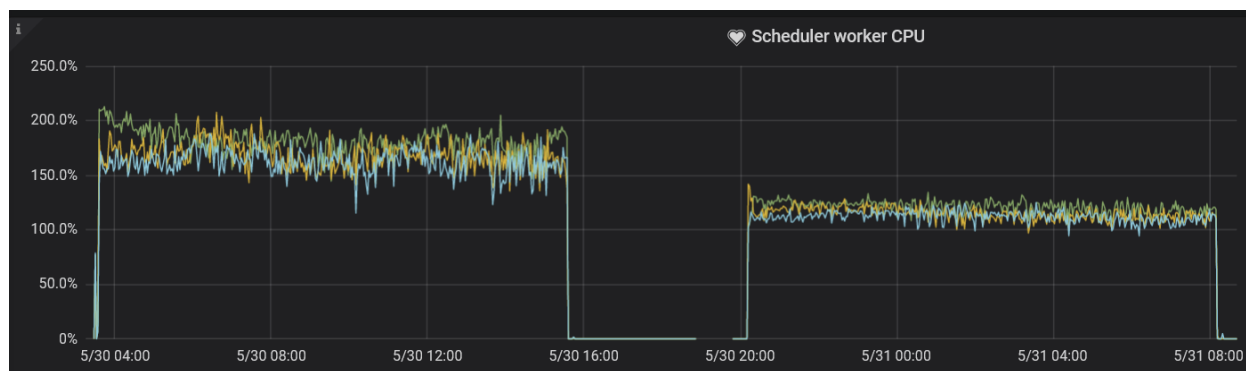
图 234: Scheduler Worker CPU
