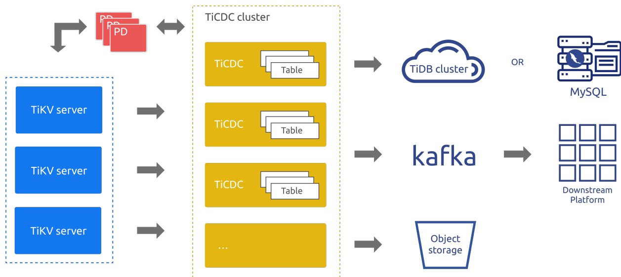
图 279: TiCDC architecture
