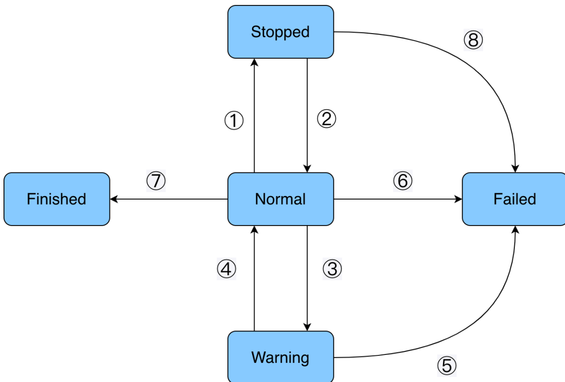
图 280: TiCDC state transfer
