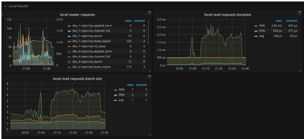
图 359: TiKV Dashboard - Local reader metrics
