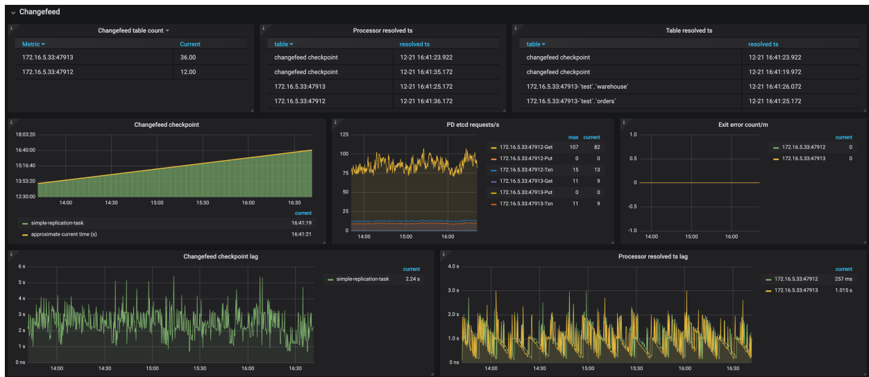
图 295: TiCDC Dashboard - Changefeed metrics 1
