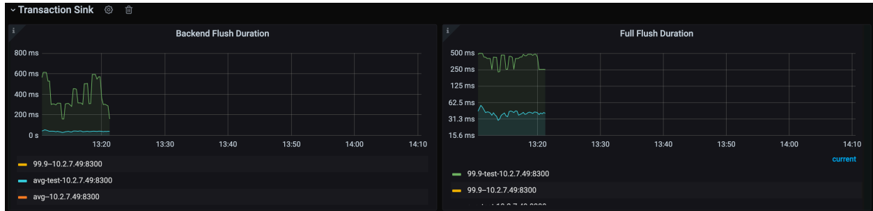
图 289: TiCDC Summary Dashboard - Transaction Sink metrics
