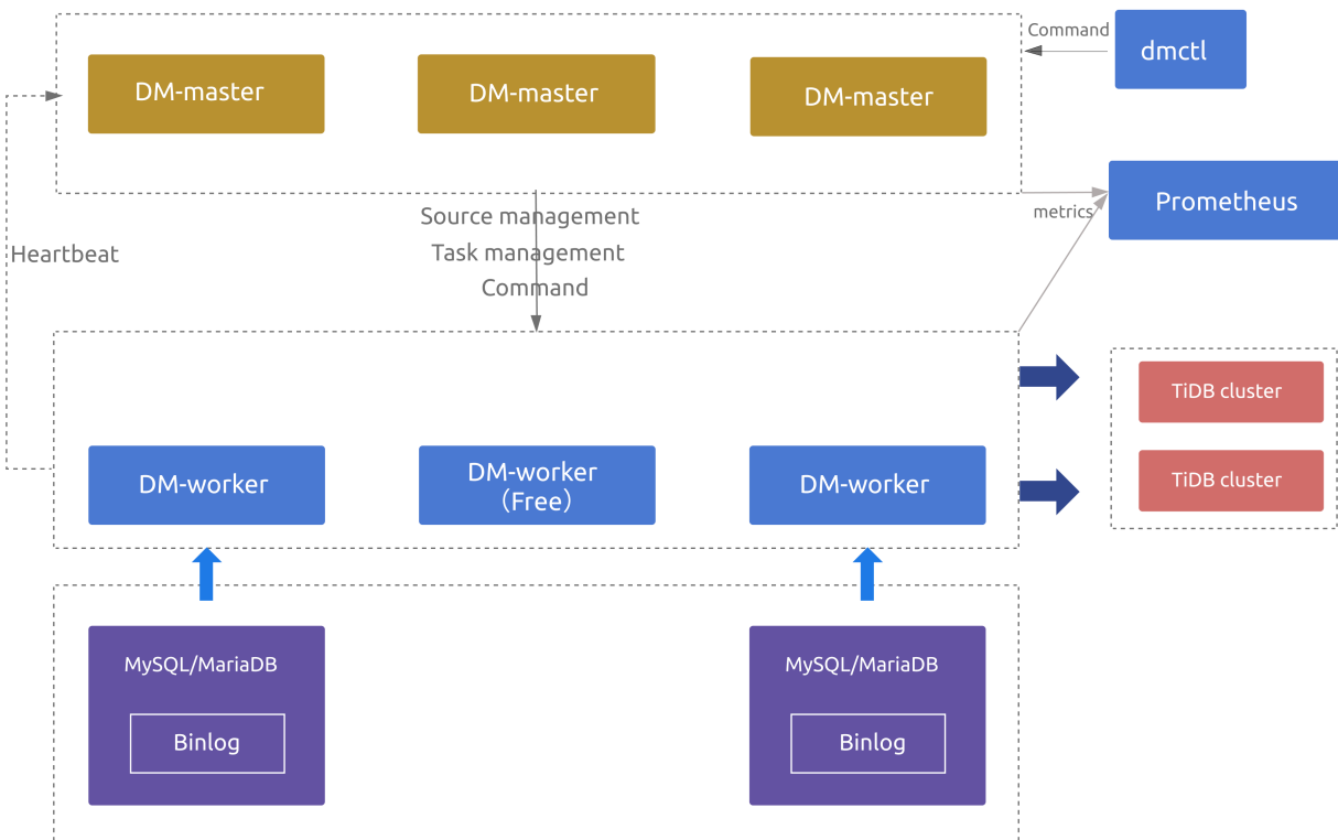
图 239: Data Migration architecture
