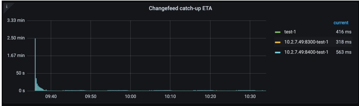
图 298: TiCDC Dashboard - Changefeed metrics 4
