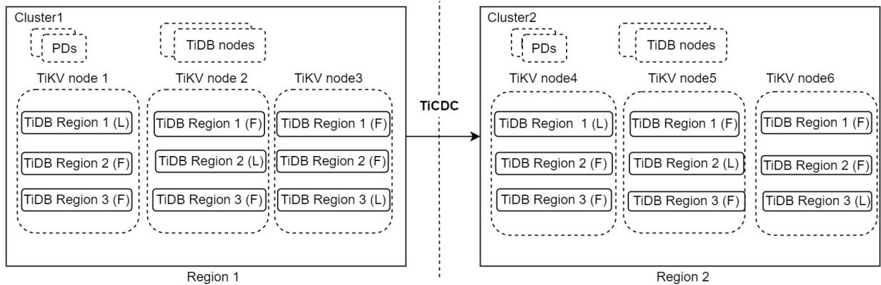
图 58: Primary-secondary cluster DR
