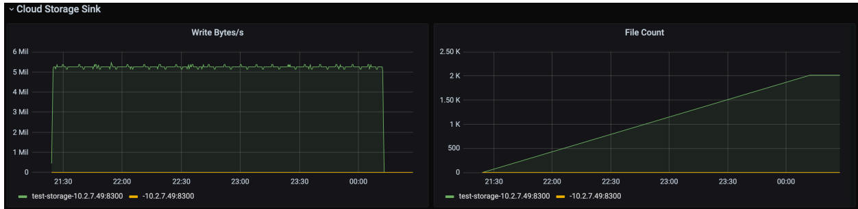
图 291: TiCDC Summary Dashboard - Transaction Sink metrics
