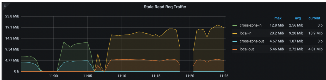
图 100: Stale Read Req Traffic
