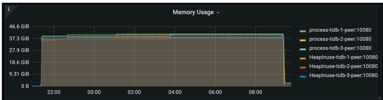
图 175: v6.1.3 workload no oom with GOMEMLIMIT
