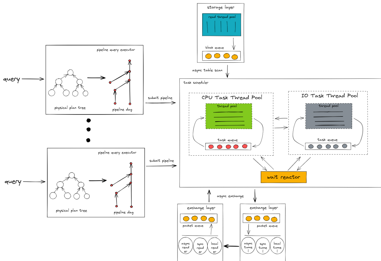
图 336: TiFlash Pipeline Model Design
