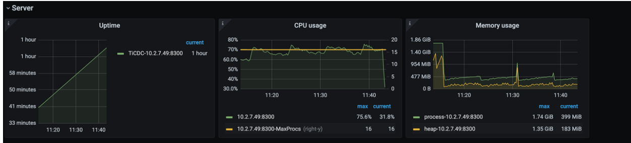
图 283: TiCDC Summary Dashboard - Server metrics
