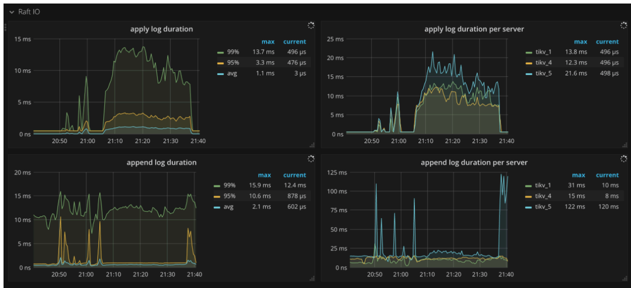
图 354: TiKV Dashboard - Raft IO metrics
