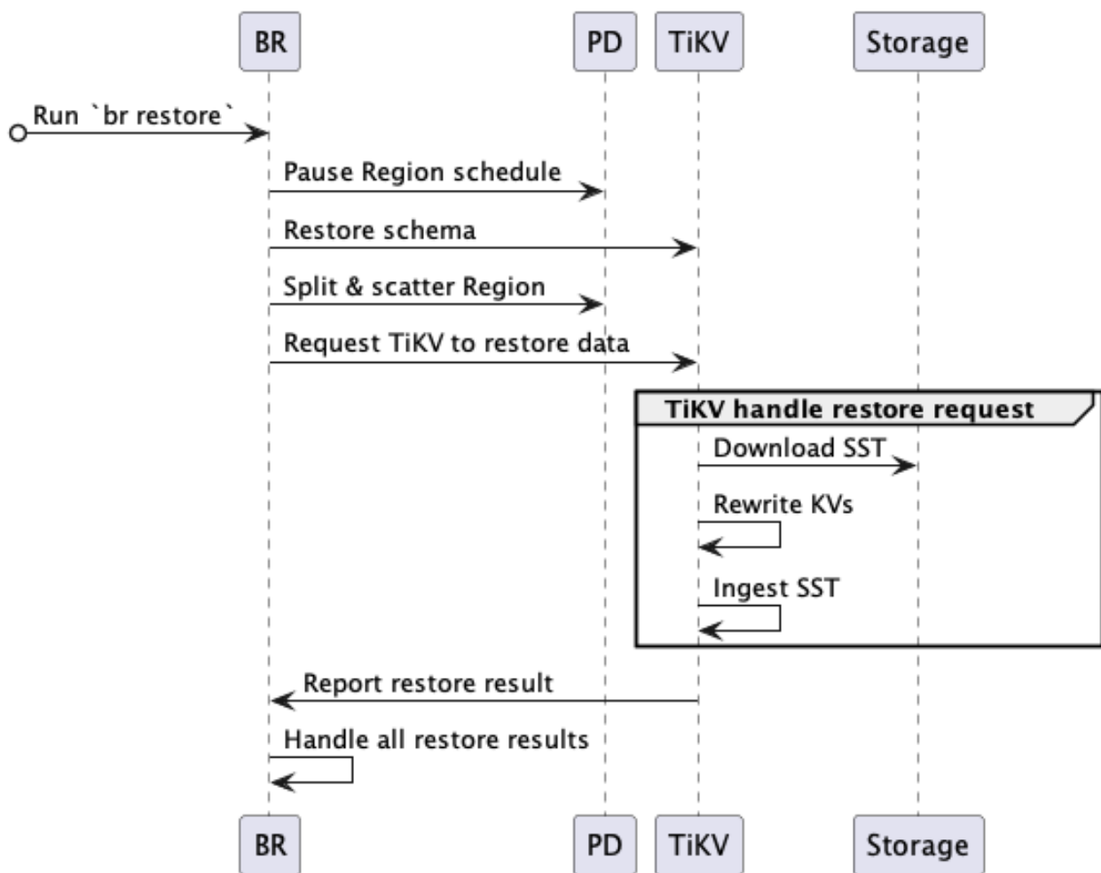
图 49: snapshot restore process design
