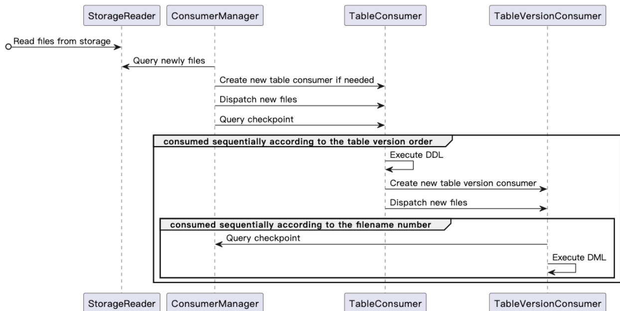
图 303: TiCDC storage consumer overview
