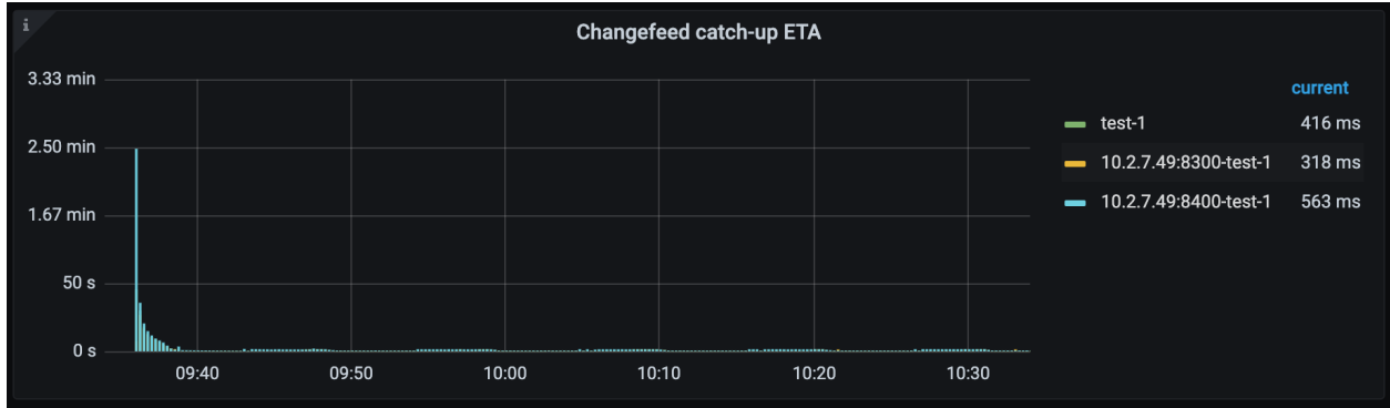
图 369: TiCDC Dashboard - Changefeed metrics 4
