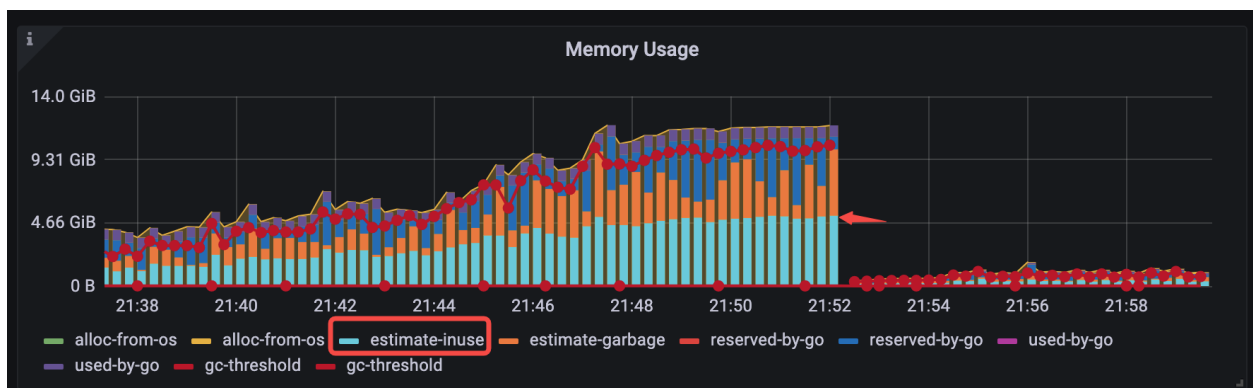
图 173: normal OOM case example
