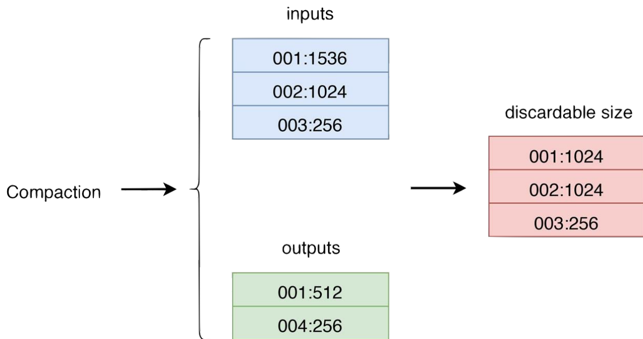
Figure 387: EventListener
