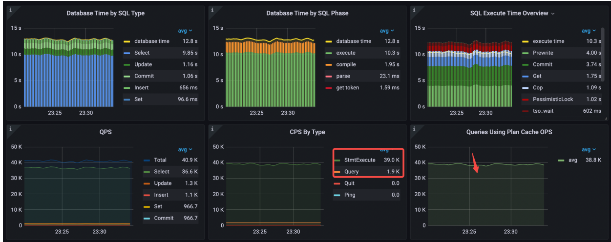
Figure 222: performance-overview-1-for-table-cache
