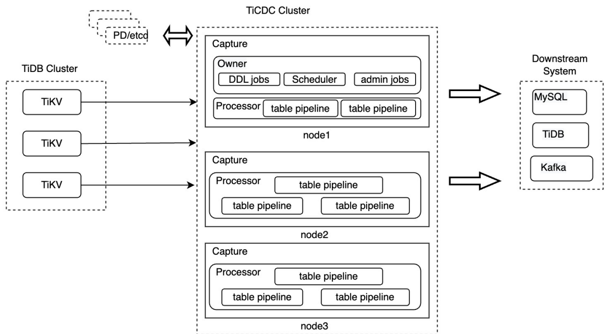
Figure 358: TiCDC architecture
