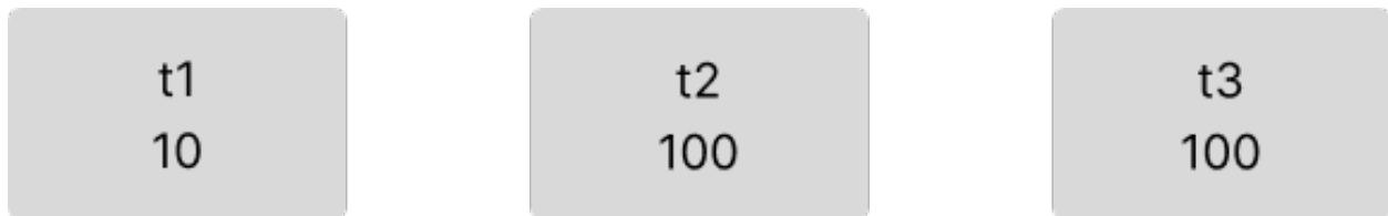
Figure 237: join-reorder-1
