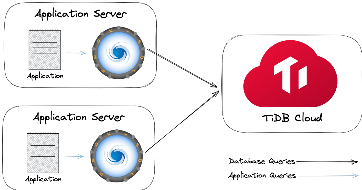
Figure 66: proxysql-client-side-tidb-cloud
