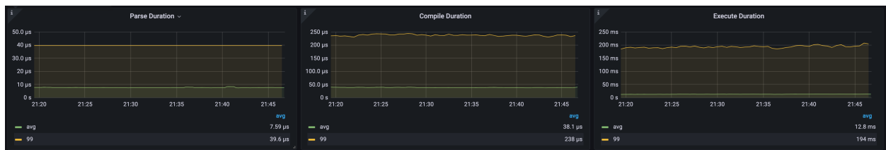
Figure 182: Execute
