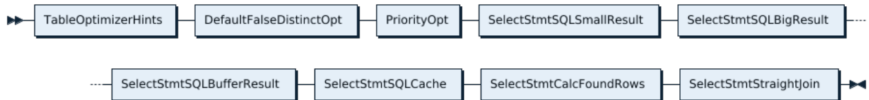
Figure 434: SelectStmtOpts
