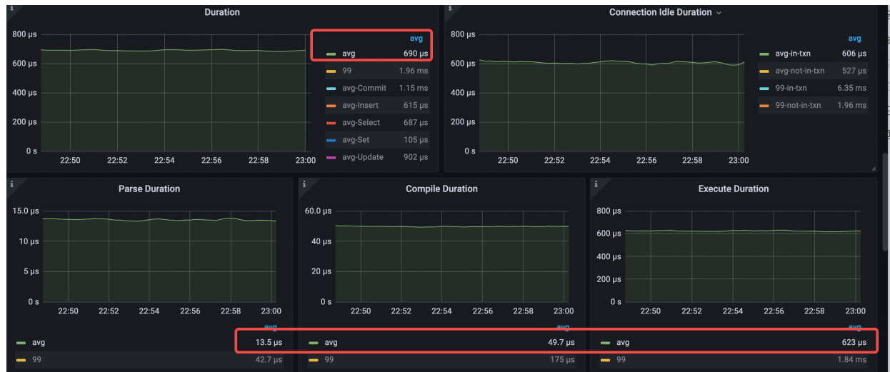
Figure 215: performance-overview-for-3-command
