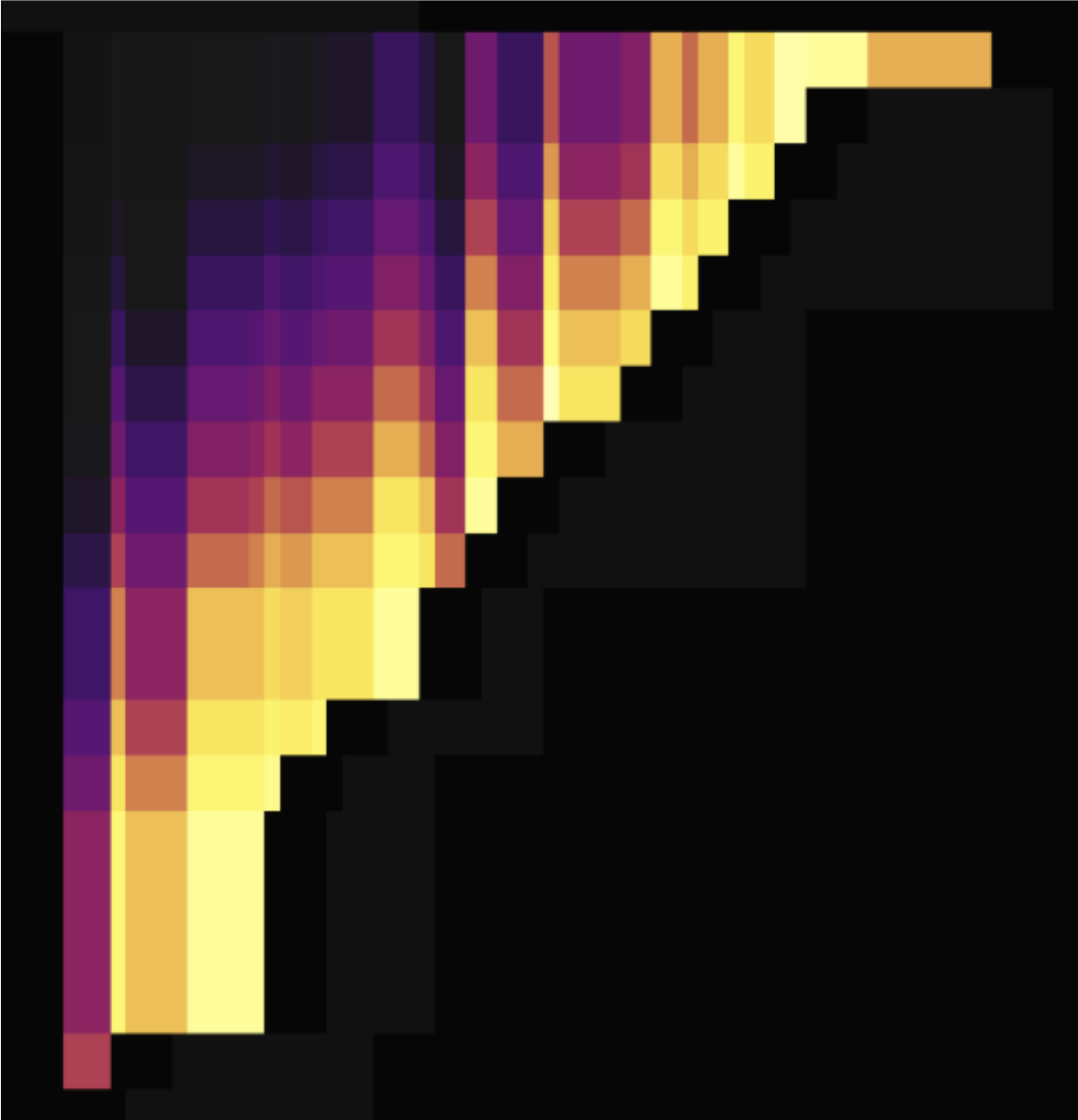
Figure 144: Dashboard Example 5
