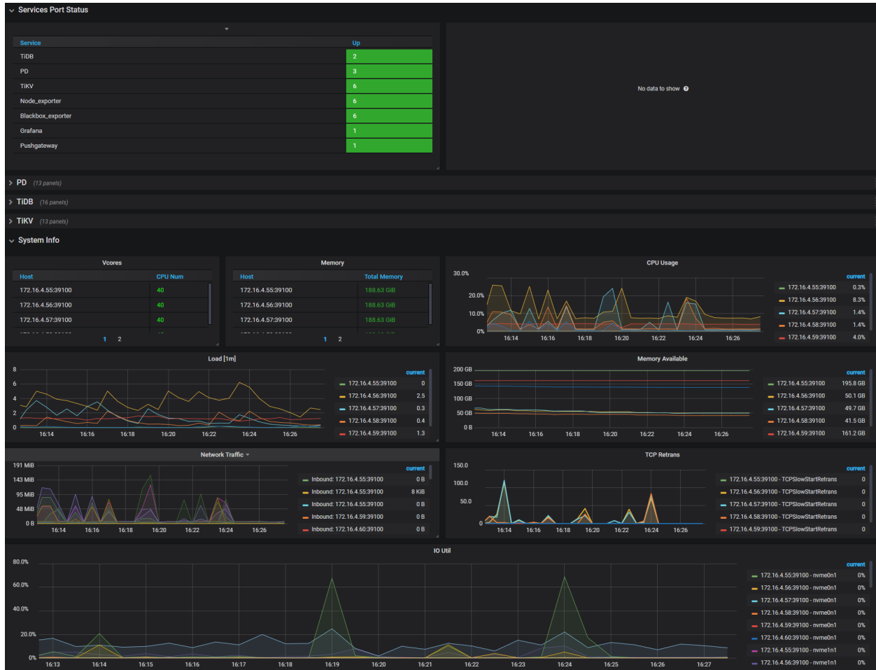
Figure 399: overview
