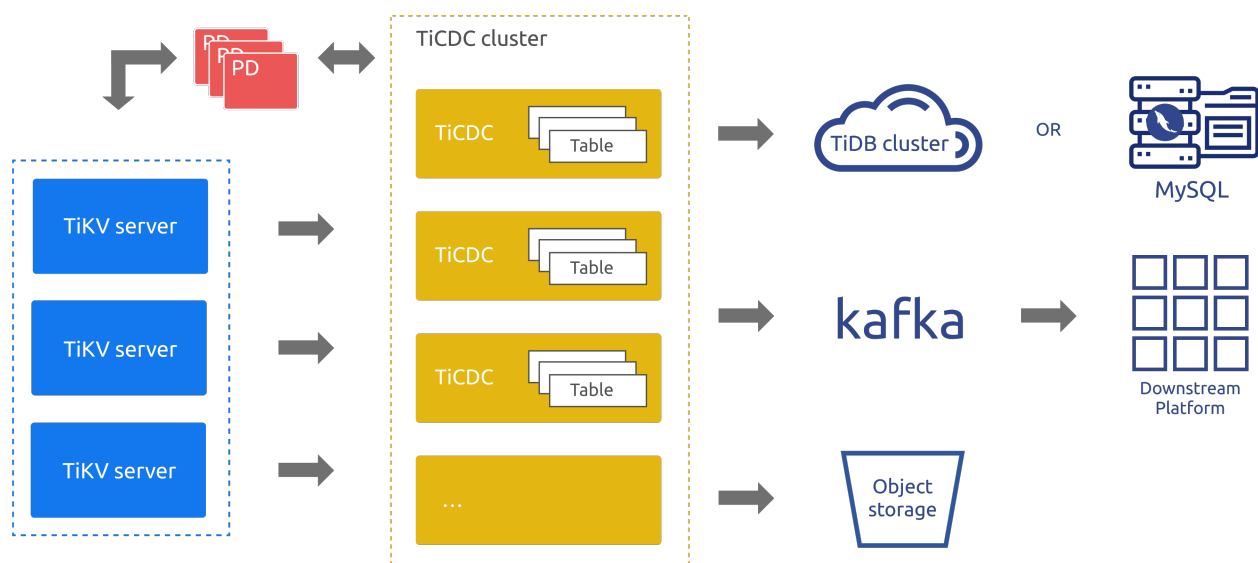
Figure 116: TiCDC architecture
