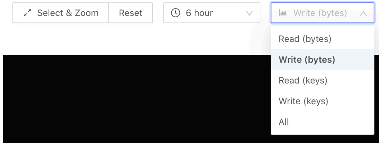
Figure 559: Select metrics
