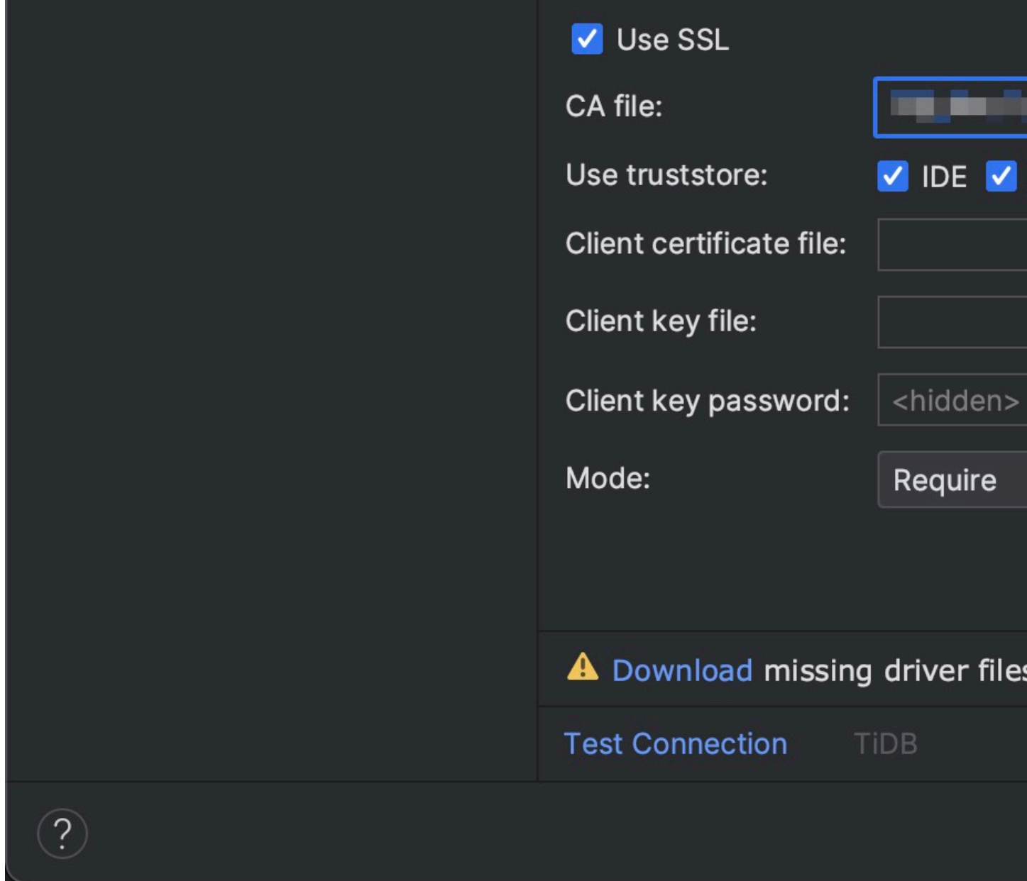
Figure 8: Configure the CA for TiDB Cloud Dedicated
