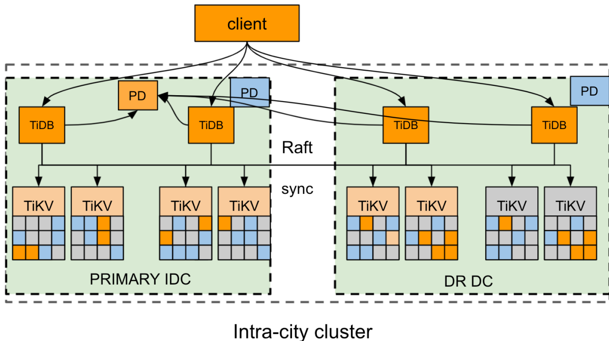
Figure 258: 2-AZ-in-1-region architecture
