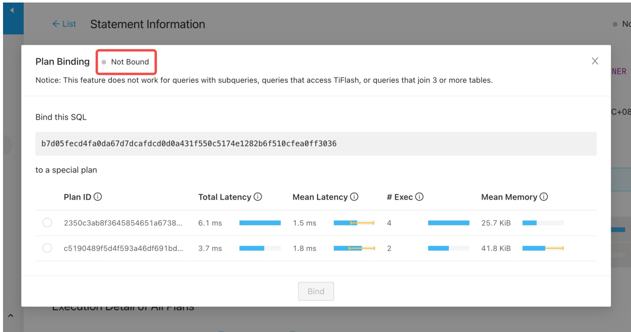
Figure 581: Fast plan binding - popup
