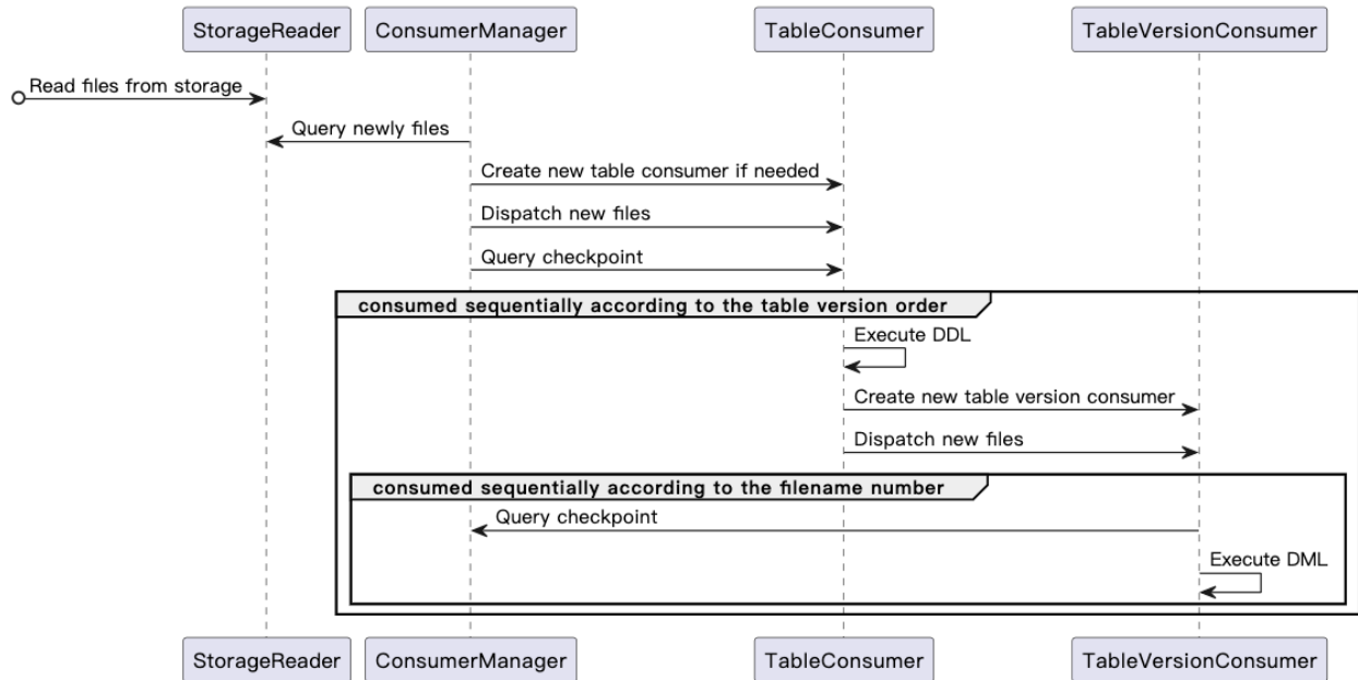
Figure 362: TiCDC storage consumer overview
