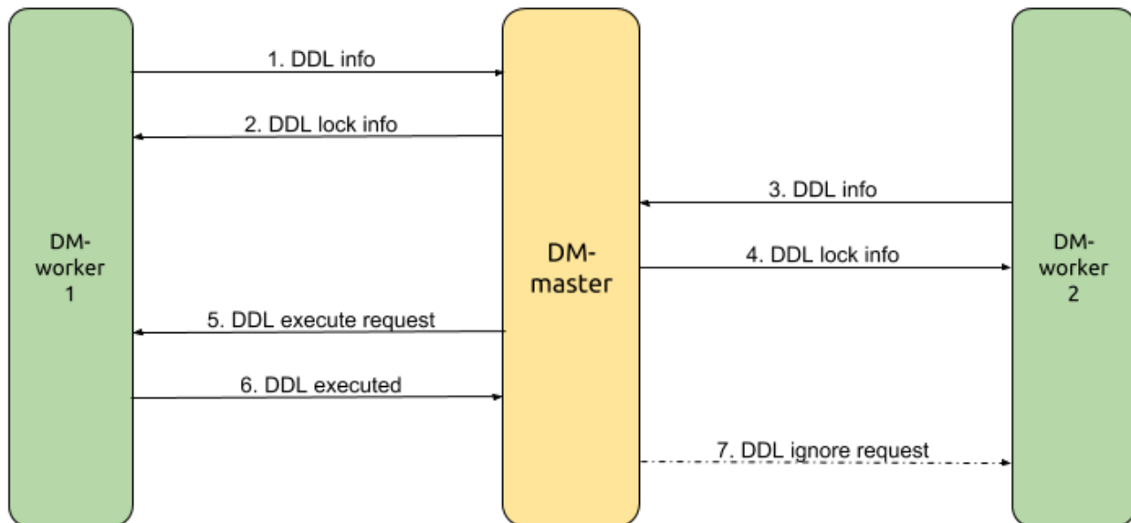
Figure 302: shard-ddl-flow
