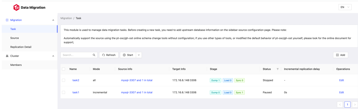
Figure 320: webui
