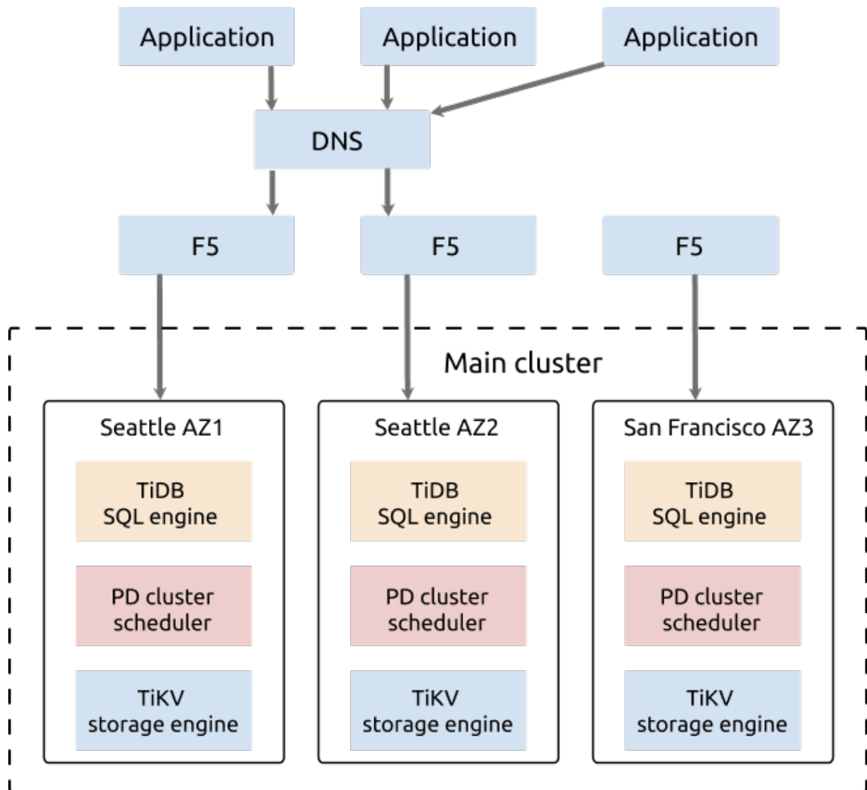
Figure 255: 3-AZ-in-2-region architecture
