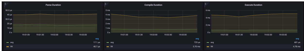
Figure 181: Compile
