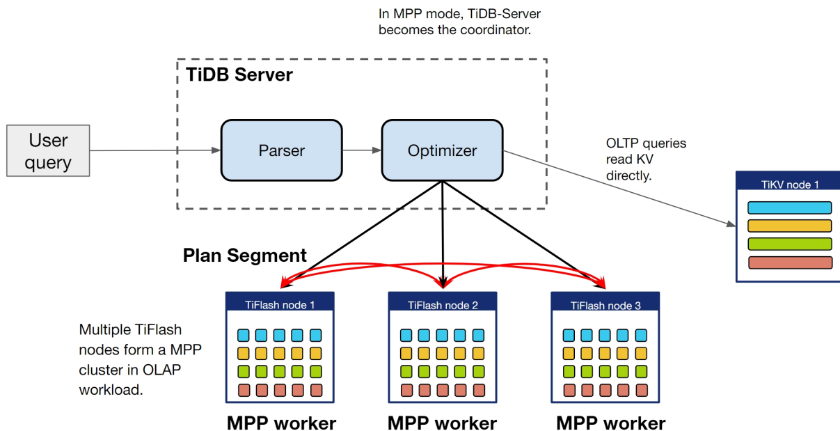
Figure 391: mpp-mode
