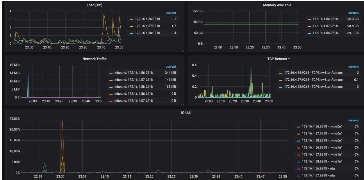
Figure 131: Overview panel
