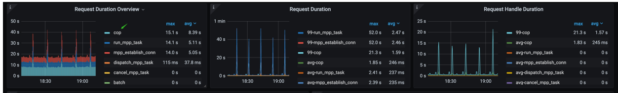
Figure 227: Cop
