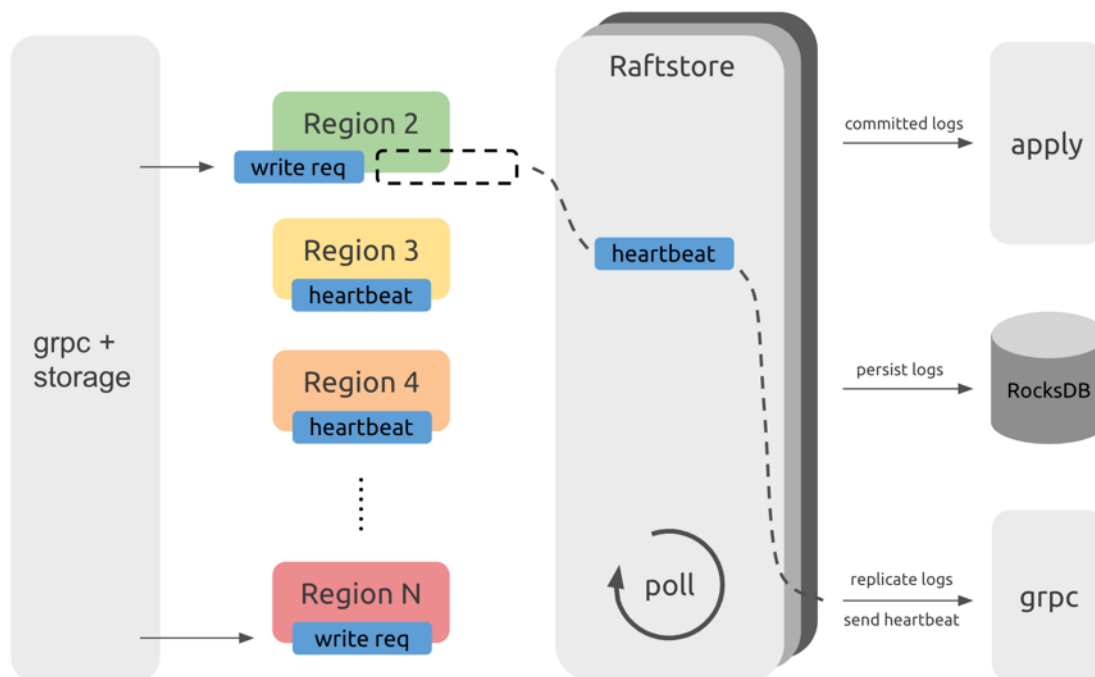
Figure 288: Raftstore Workflow
