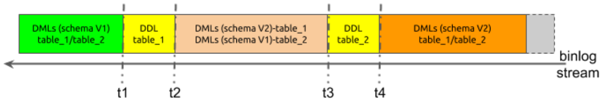
Figure 303: shard-ddl-example-2
