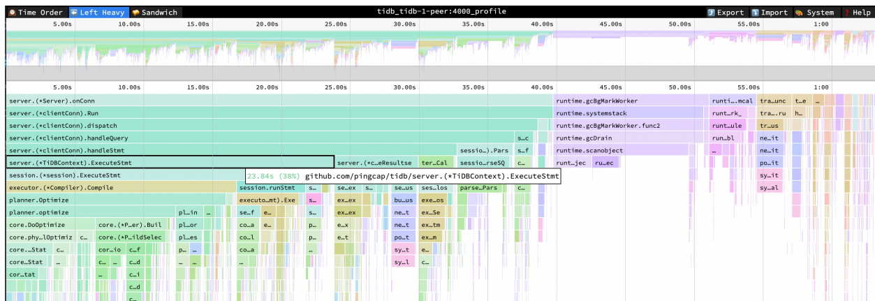
Figure 196: flame-graph-for-query-interface
