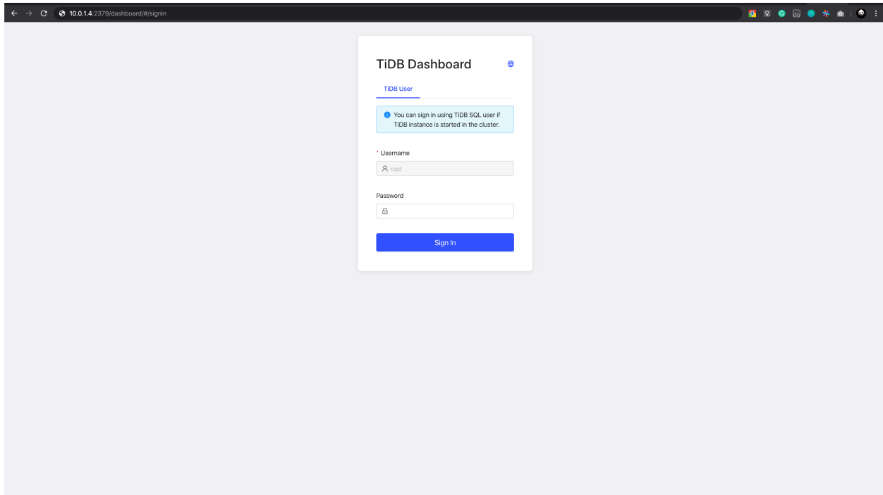
Figure 91: TiDB-Dashboard
