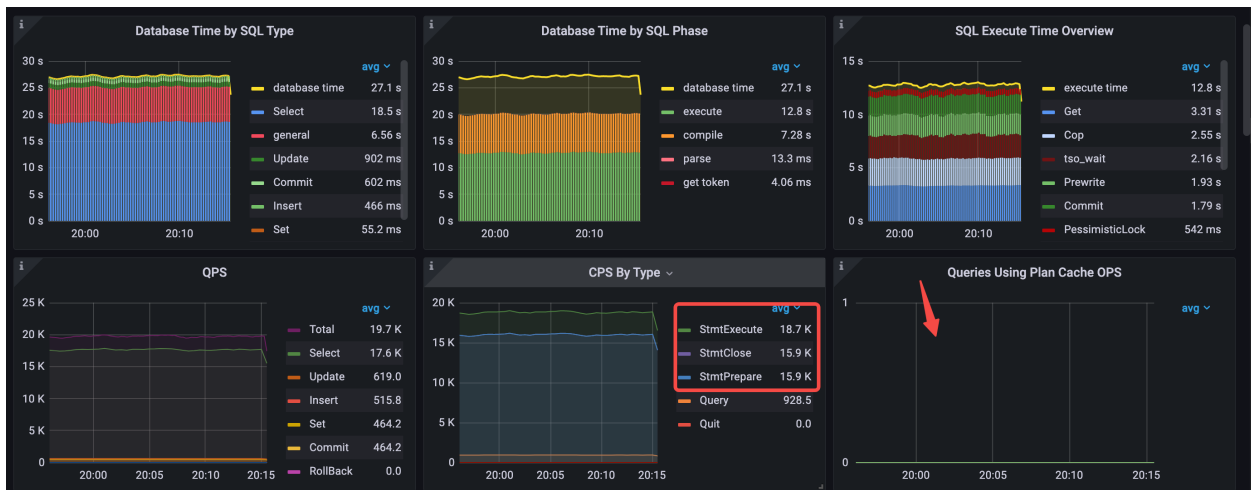
Figure 205: performance-overview-1-for-PrepStmts
