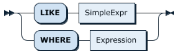
Figure 482: ShowLikeOrWhereOpt
