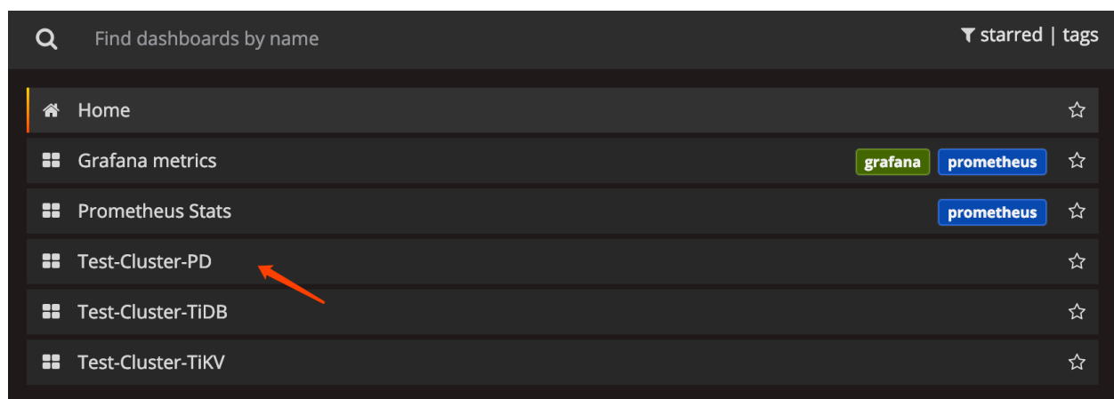
Figure 137: view dashboard
