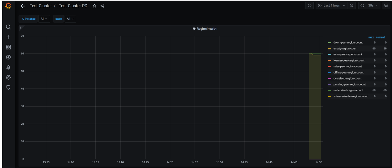
Figure 128: Region panel
