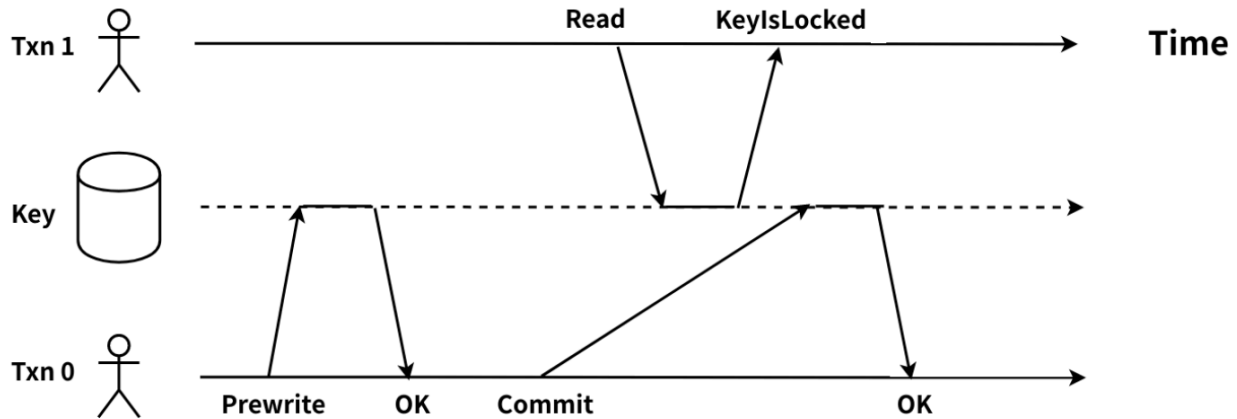
Figure 151: read-write conflict
