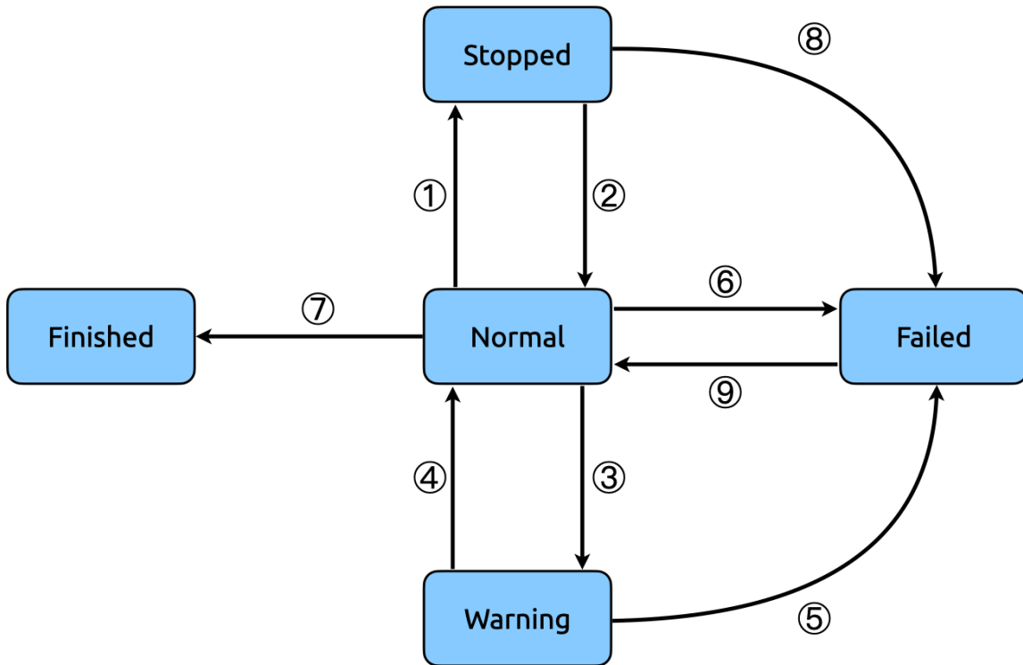
图 286: TiCDC state transfer
