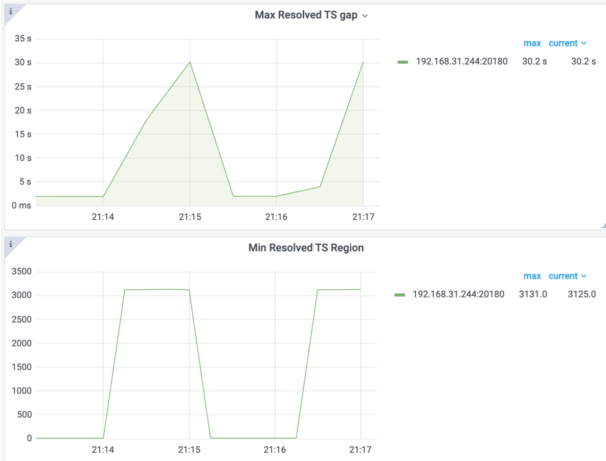
图 107: Example: Max Resolved TS gap
