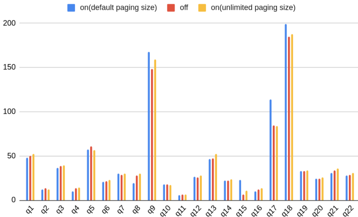
图 349: Paging size impact on TPC-H
