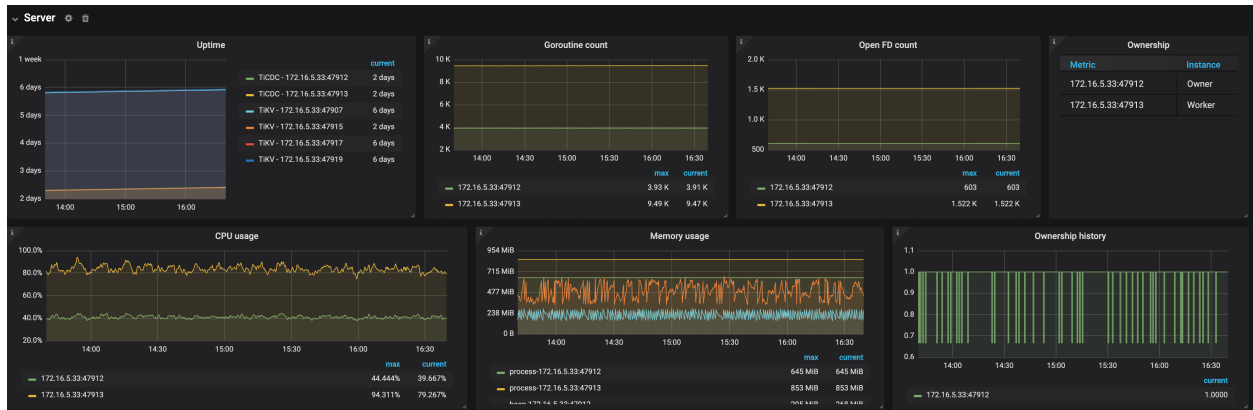
图 300: TiCDC Dashboard - Server metrics
