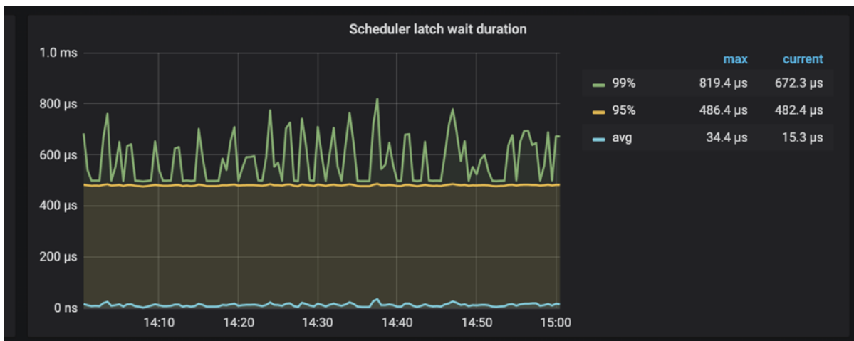
图 386: Scheduler latch wait duration
