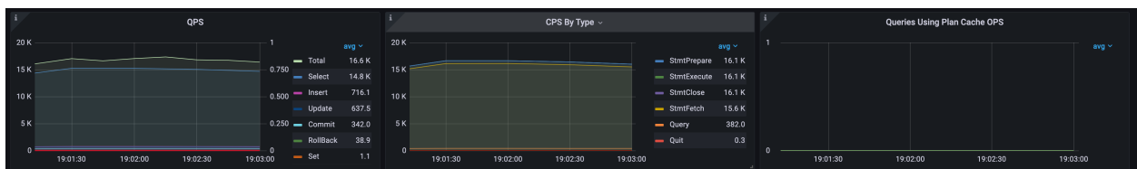
图 117: OLTP-Prepared
