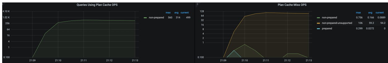
图 194: non-prepared-unsupported
