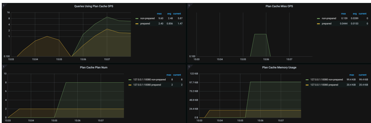
图 195: non-prepared-plan-cache
