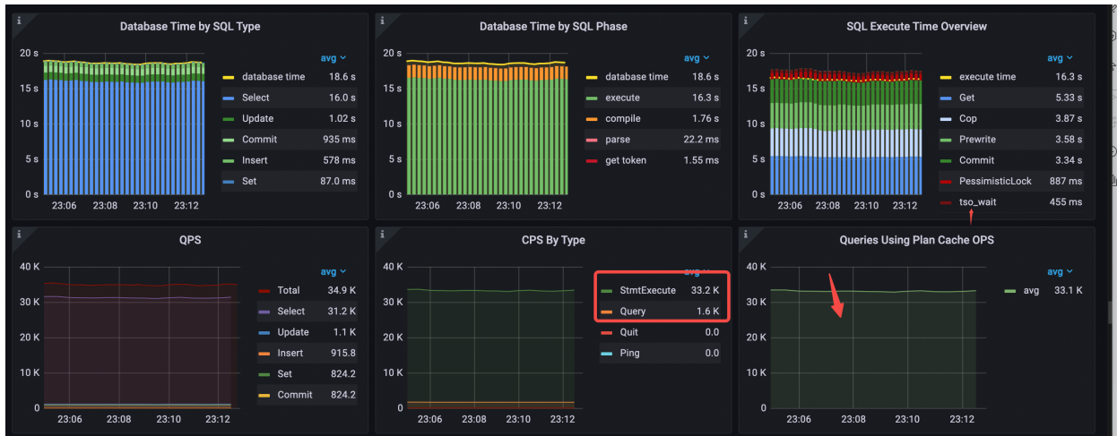
图 165: performance-overview-1-for-rc-read
