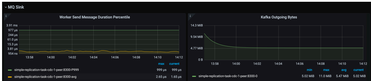
图 296: TiCDC Summary Dashboard - Transaction Sink metrics
